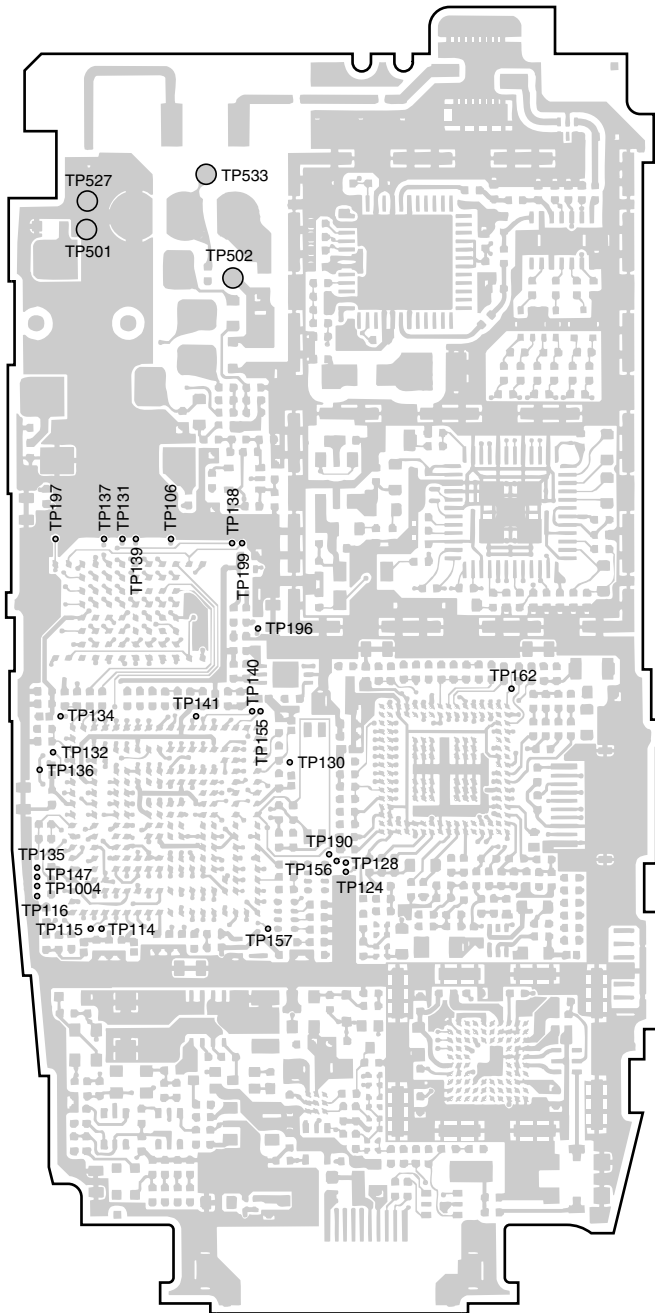
Figure 75 TEST POINT
