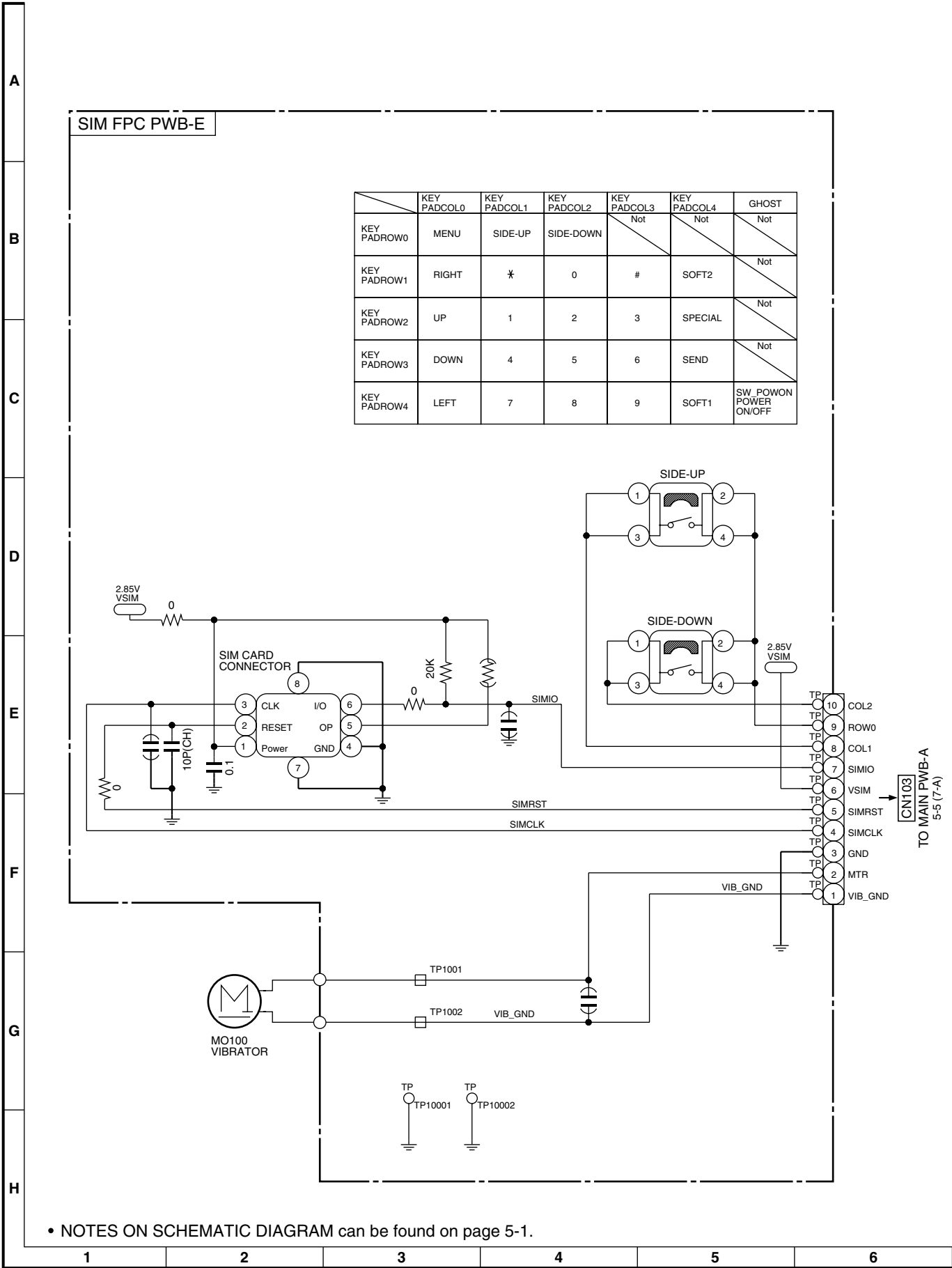
Figure 9 SCHEMATIC DIAGRAM (5/6)
