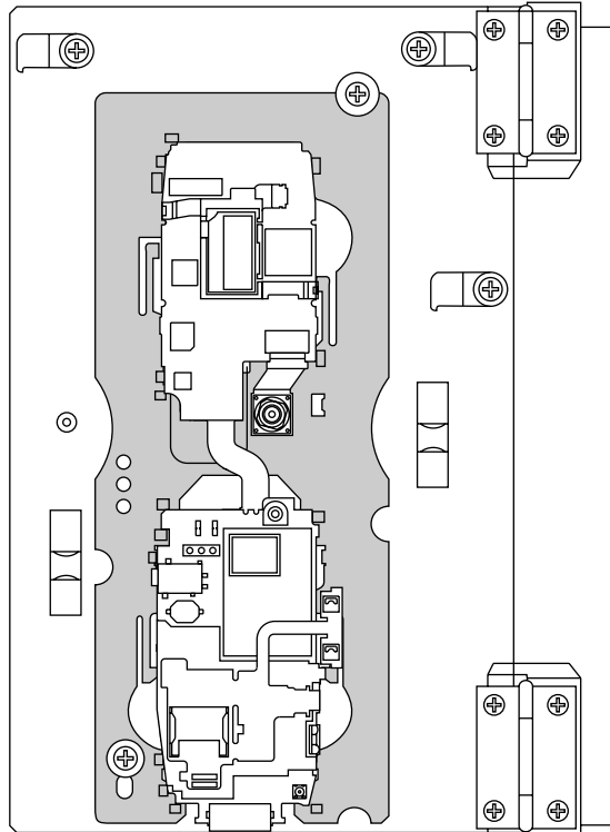
Figure 51 PWB installation
