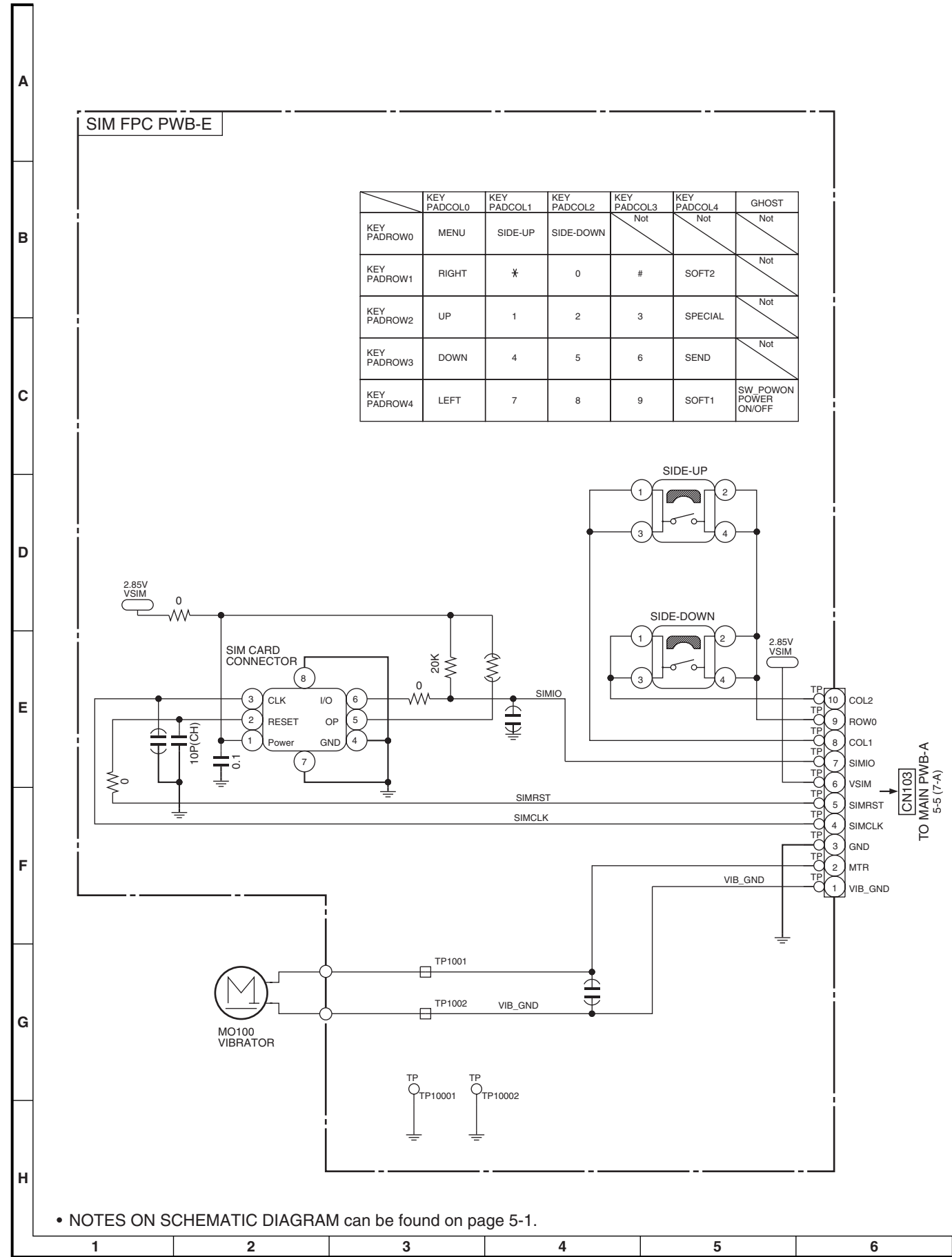
Figure 9 SCHEMATIC DIAGRAM (5/6)
