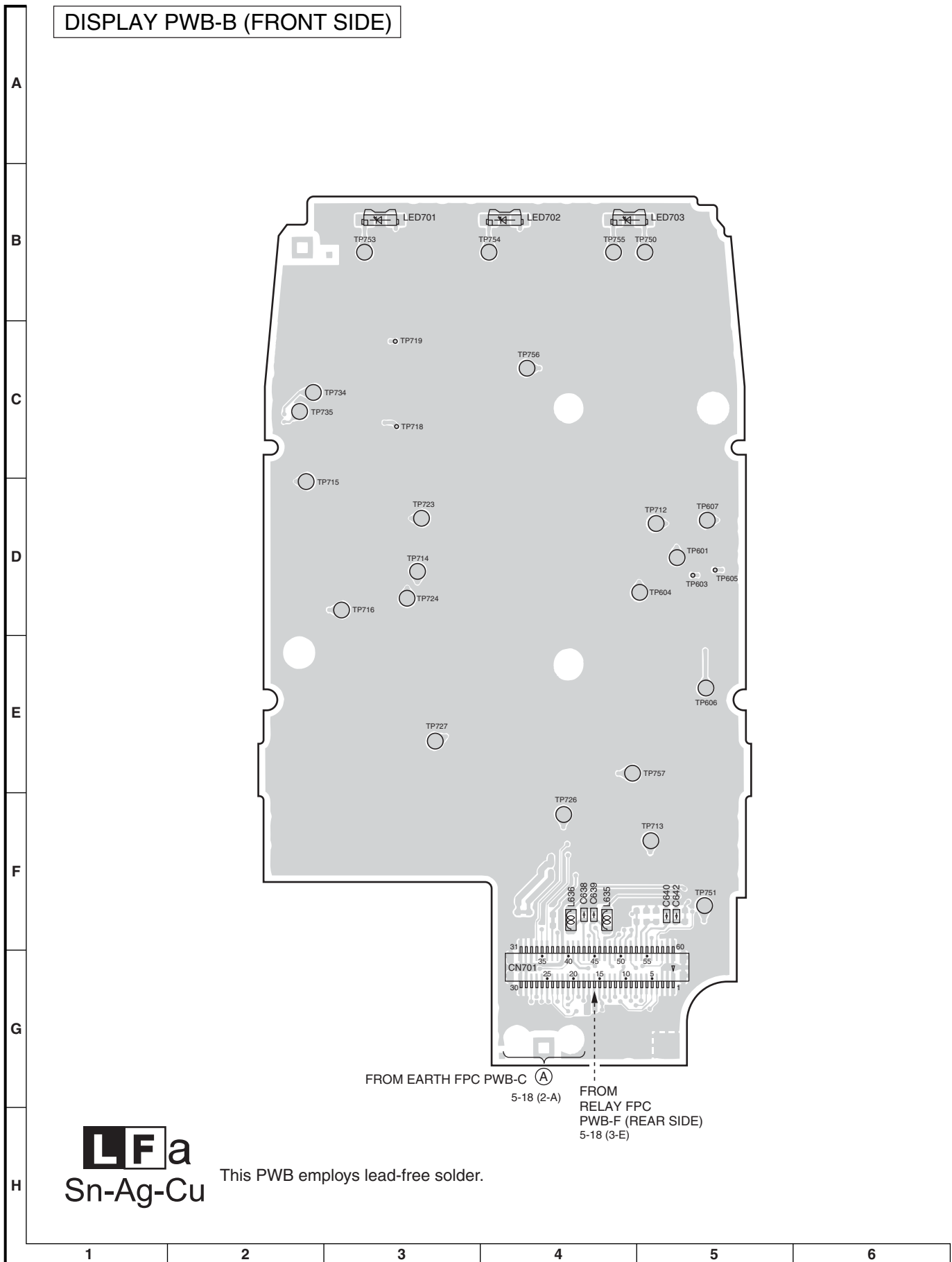
Figure 7 WIRING SIDE P.W.BOARD (3/5)
