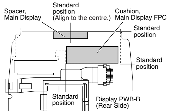
[Spacer, Main Display/Cushion, Main Display FPC]
