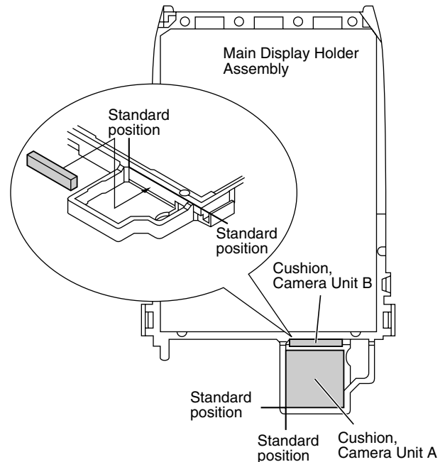
[Cushion, Camera Unit A/Cushion, Camera Unit B]
