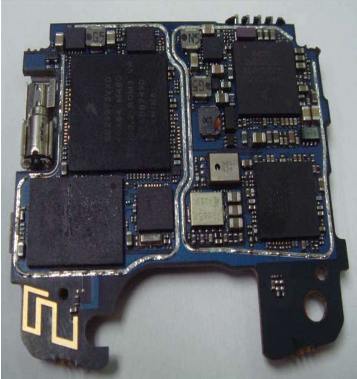
Photograph 9-1: Rear side view of radio PC Board, without shields.
