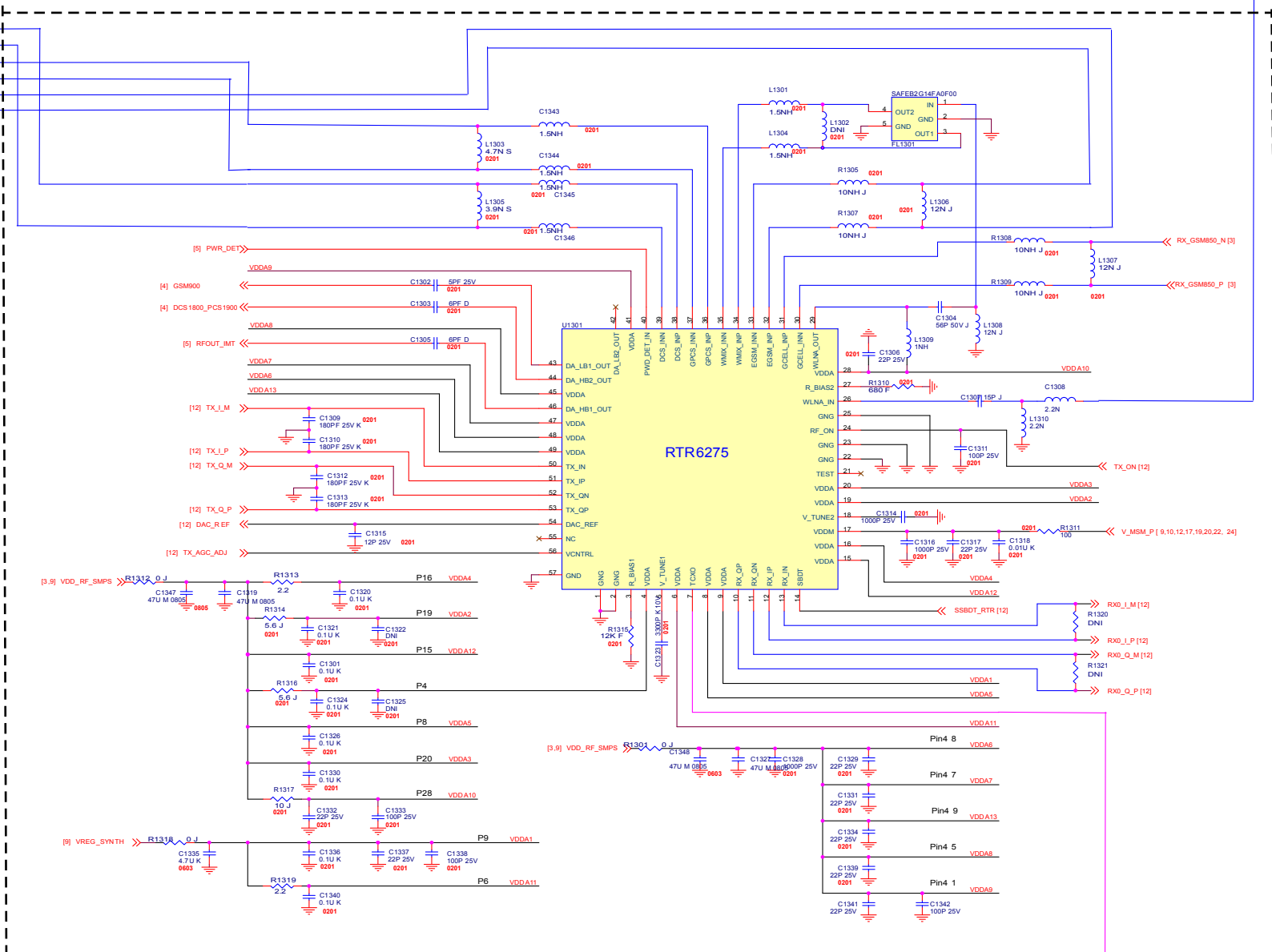
Qualcomm RTR6275 RF Transceiver
