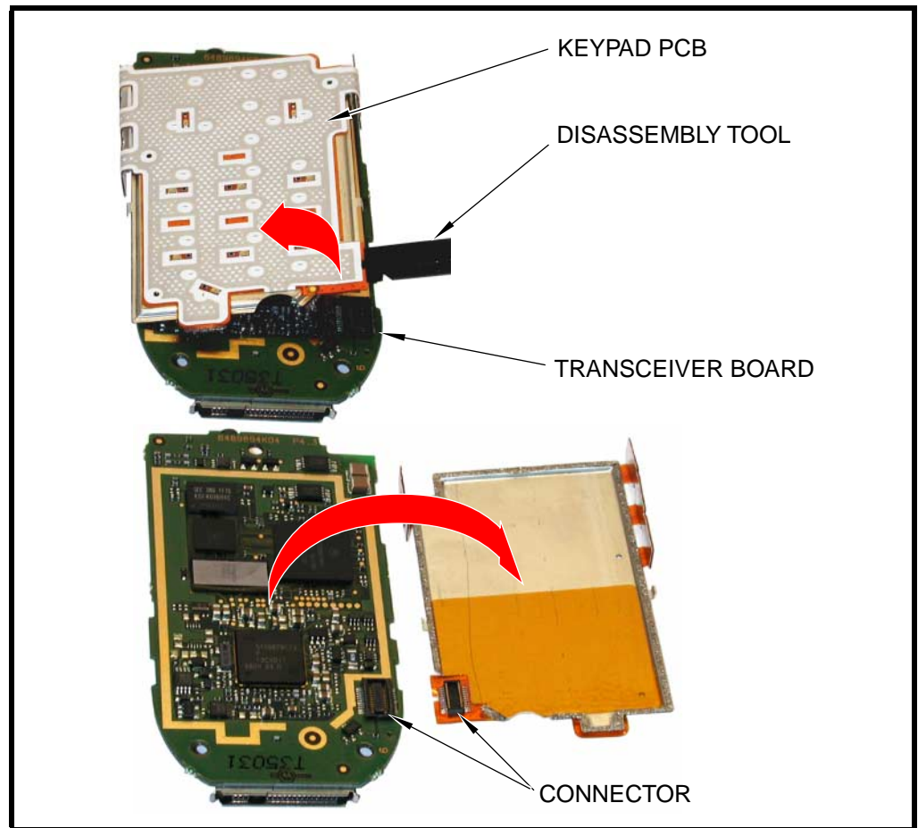
Figure 14. Removing the keypad PCB
