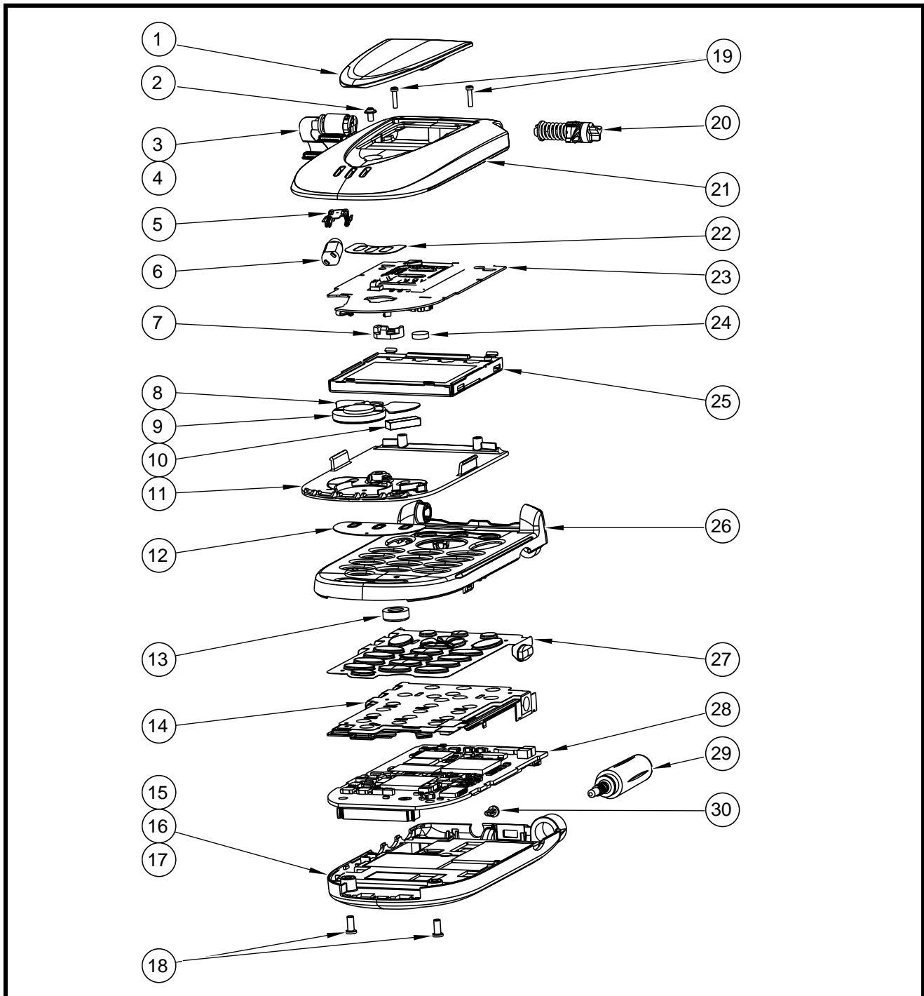
Figure 29. Exploded view diagram
