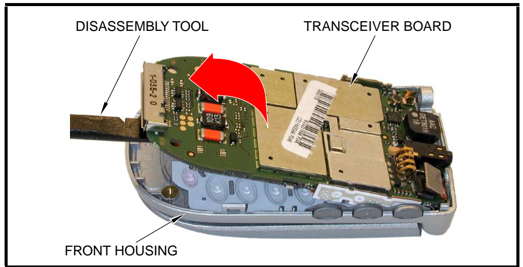
Figure 13. Removing the transceiver board assembly
