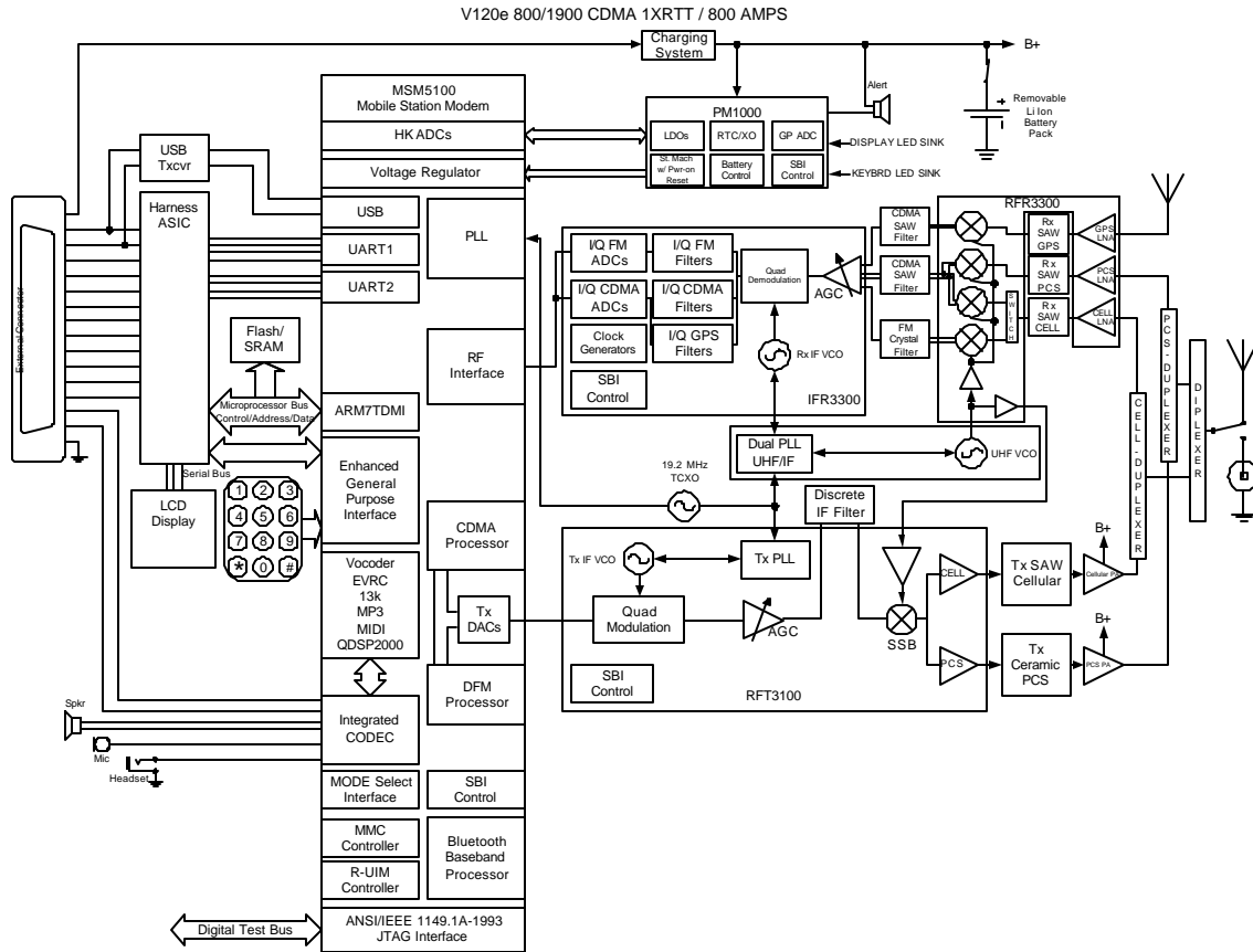
Figure 1: Motorola MSM5100 System Block Diagram
