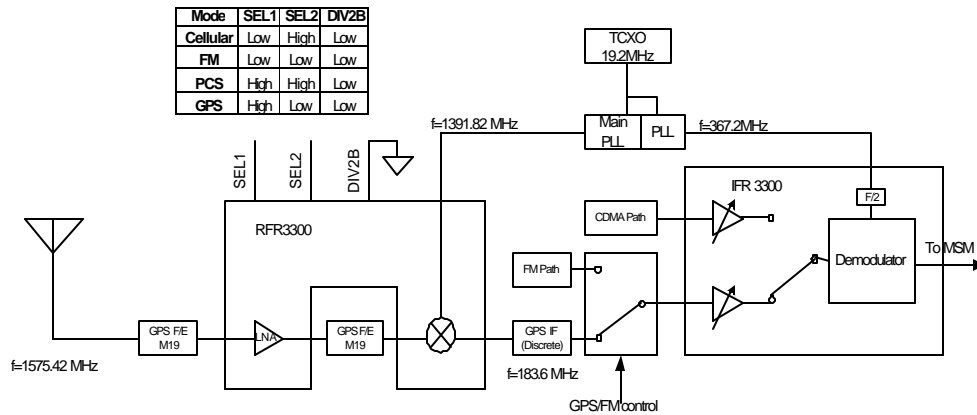
Block Diagram for GPS
