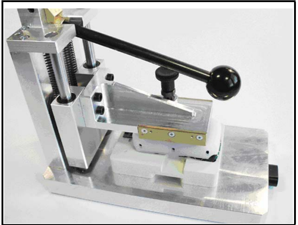
Figure 32. El Mylar Press Fixture Closed
