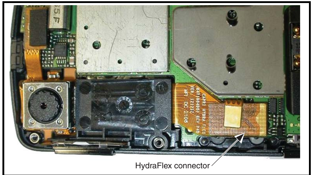
Figure 15. Disconnecting the Flex From the Transceiver Board
