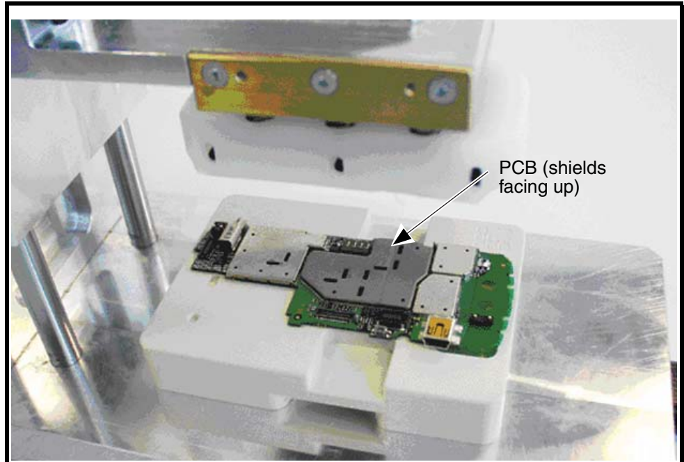
Figure 31. PCB Alignment
