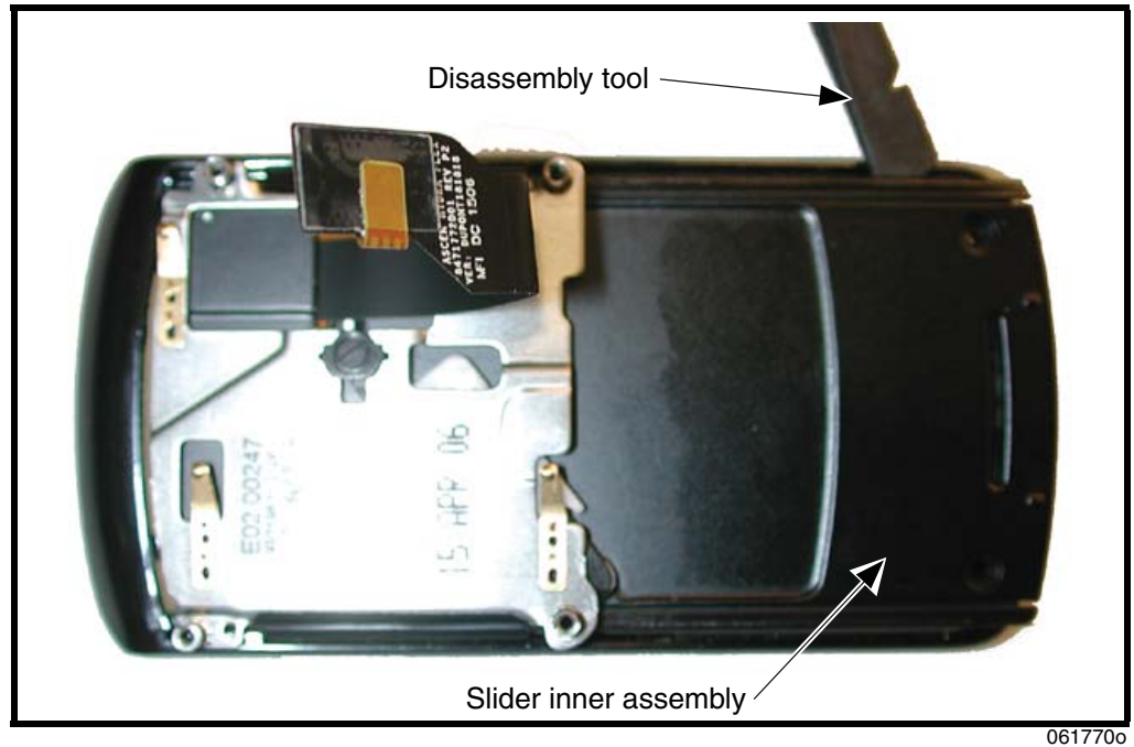
Figure 25. Removing the Slider Assembly Screws
