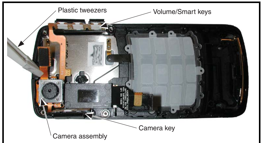
Figure 19. Removing the Camera Assembly
