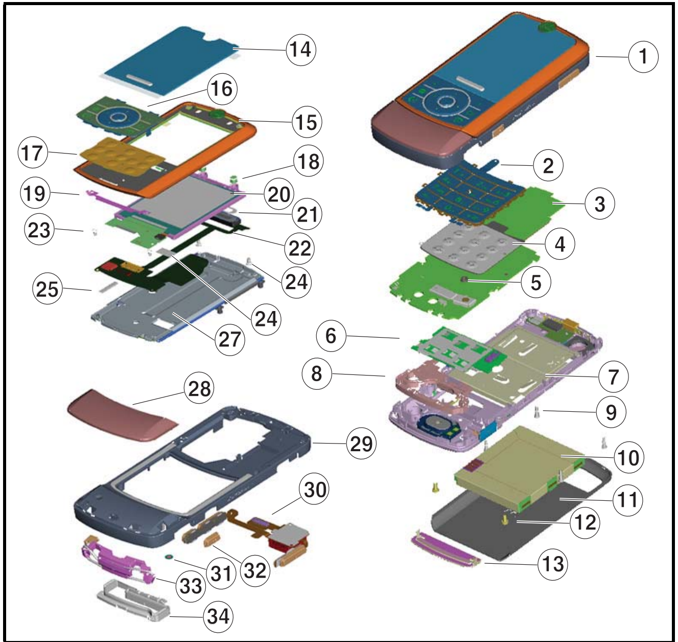
Figure 34. Exploded View Diagram (Sheet 1)
