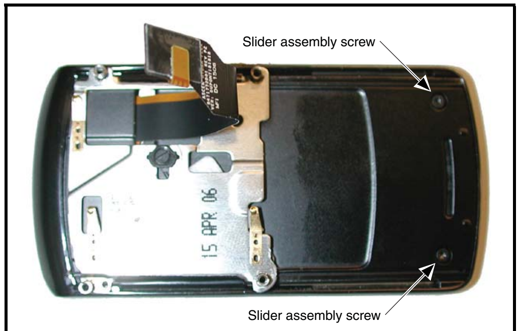
Figure 24. Removing the Slider Assembly Screws
