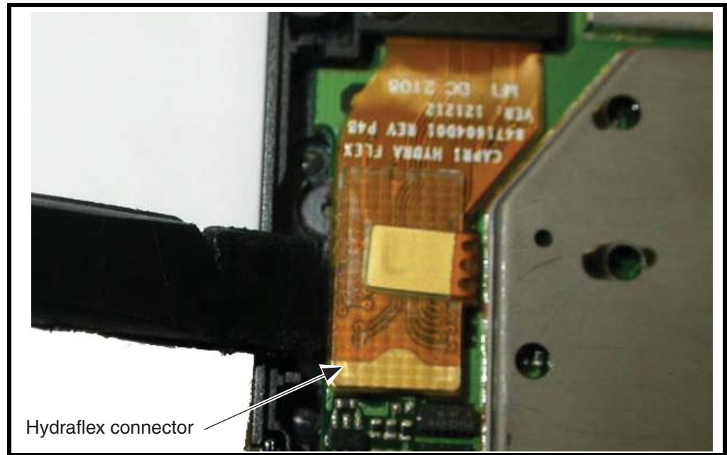
Figure 16. Disconnecting the Hydraflex Connector From the Transceiver Board
