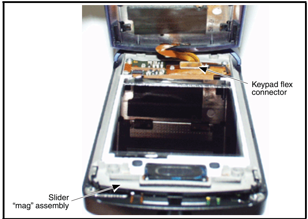
Figure 26. Removing the Keypad Flex Connector
