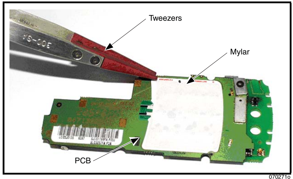
Figure 29. Removing the Keypad Mylar
