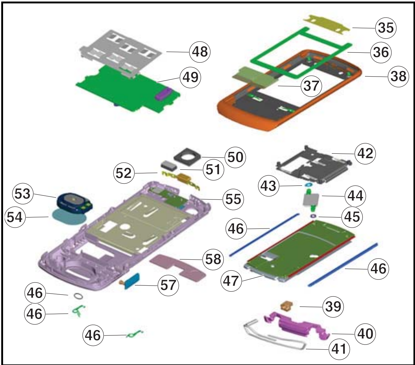
Figure 35. Exploded View Diagram (Sheet 2)
