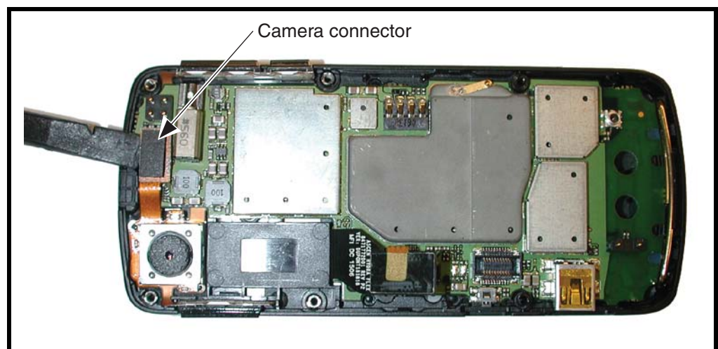
Figure 17. Removing the Camera Connector
