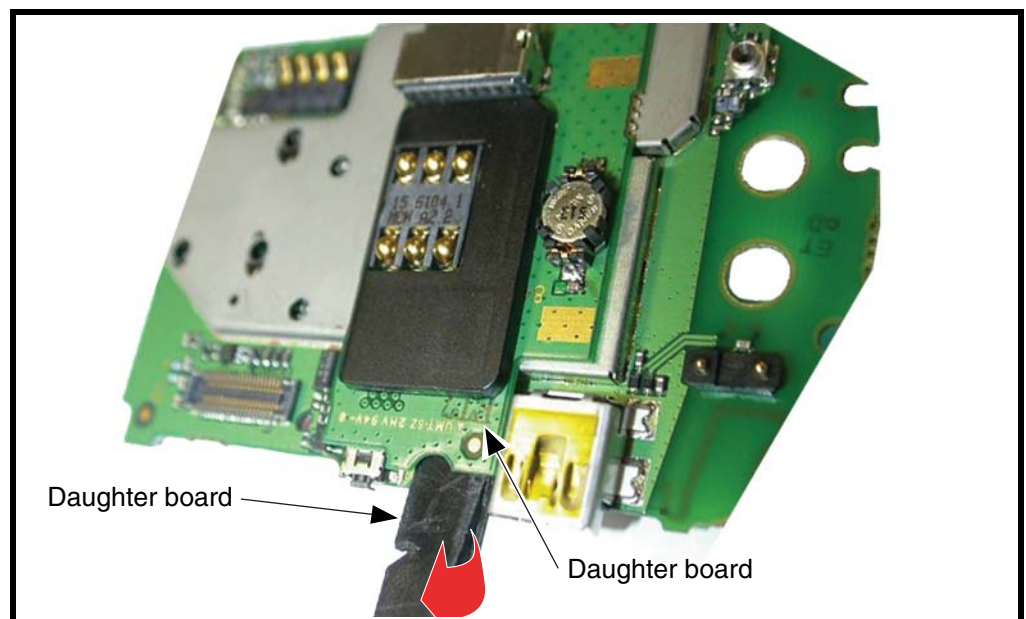
Figure 14. Removing the Daughter Board Assembly
