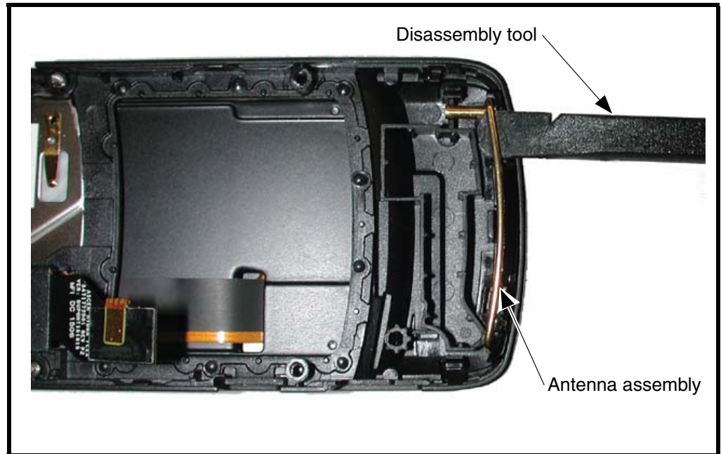
Figure 21. Removing the Antenna
