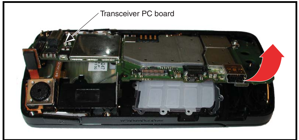
Figure 18. Removing the Transceiver PC Board Assembly
