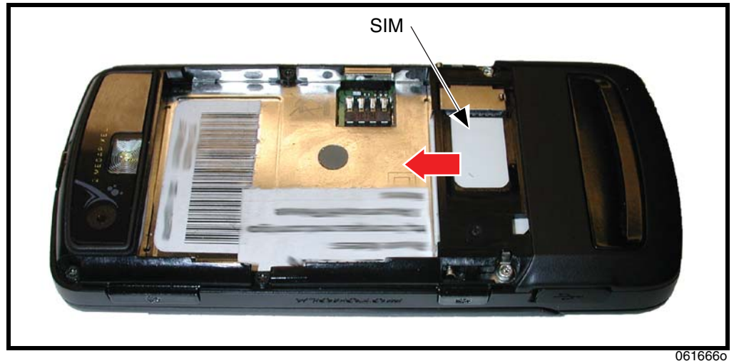
Figure 8. Removing the SIM
