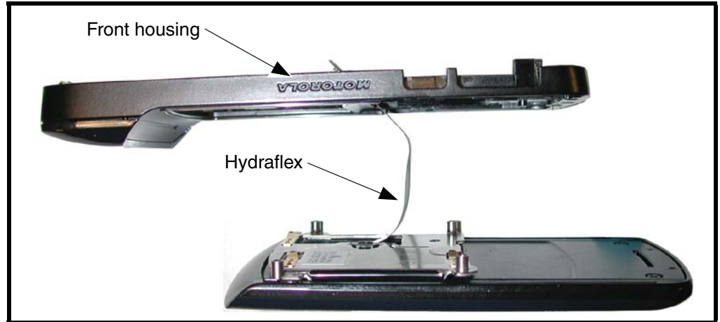
Figure 23. Removing the Front Housing
