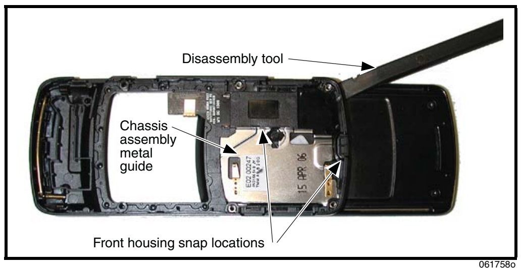
Figure 22. Removing the Front Housing Snaps
