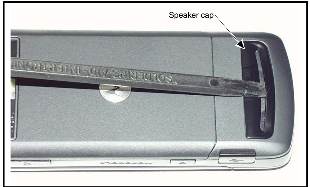
Figure 12. Removing the Speaker Cap
