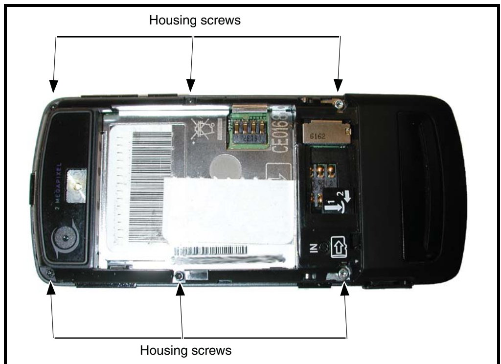
Figure 9. Removing the Rear Housing Screws
