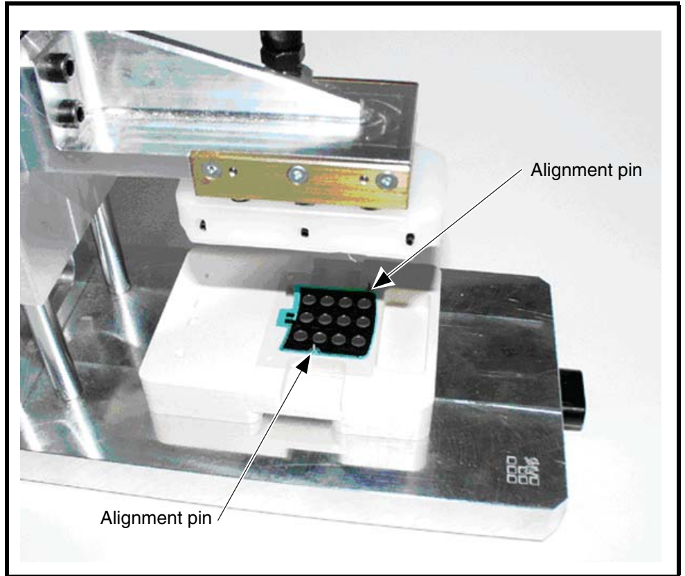
Figure 30. Keypad Mylar Alignment
