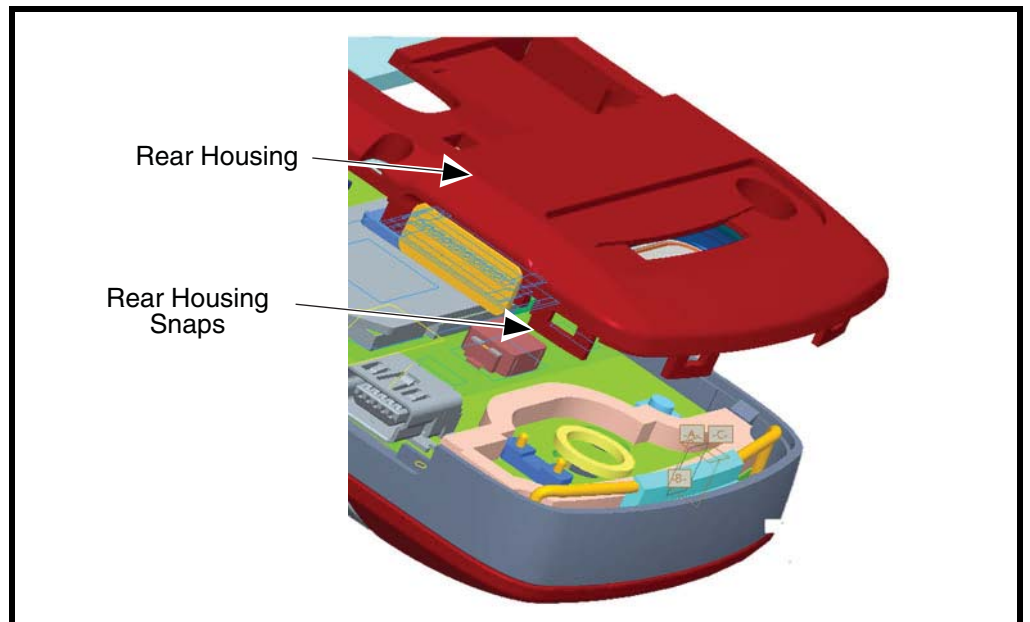
Figure 11. Removing the Rear Housing
