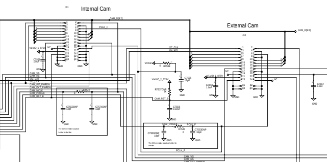
2.0 MP CONNECTOR
