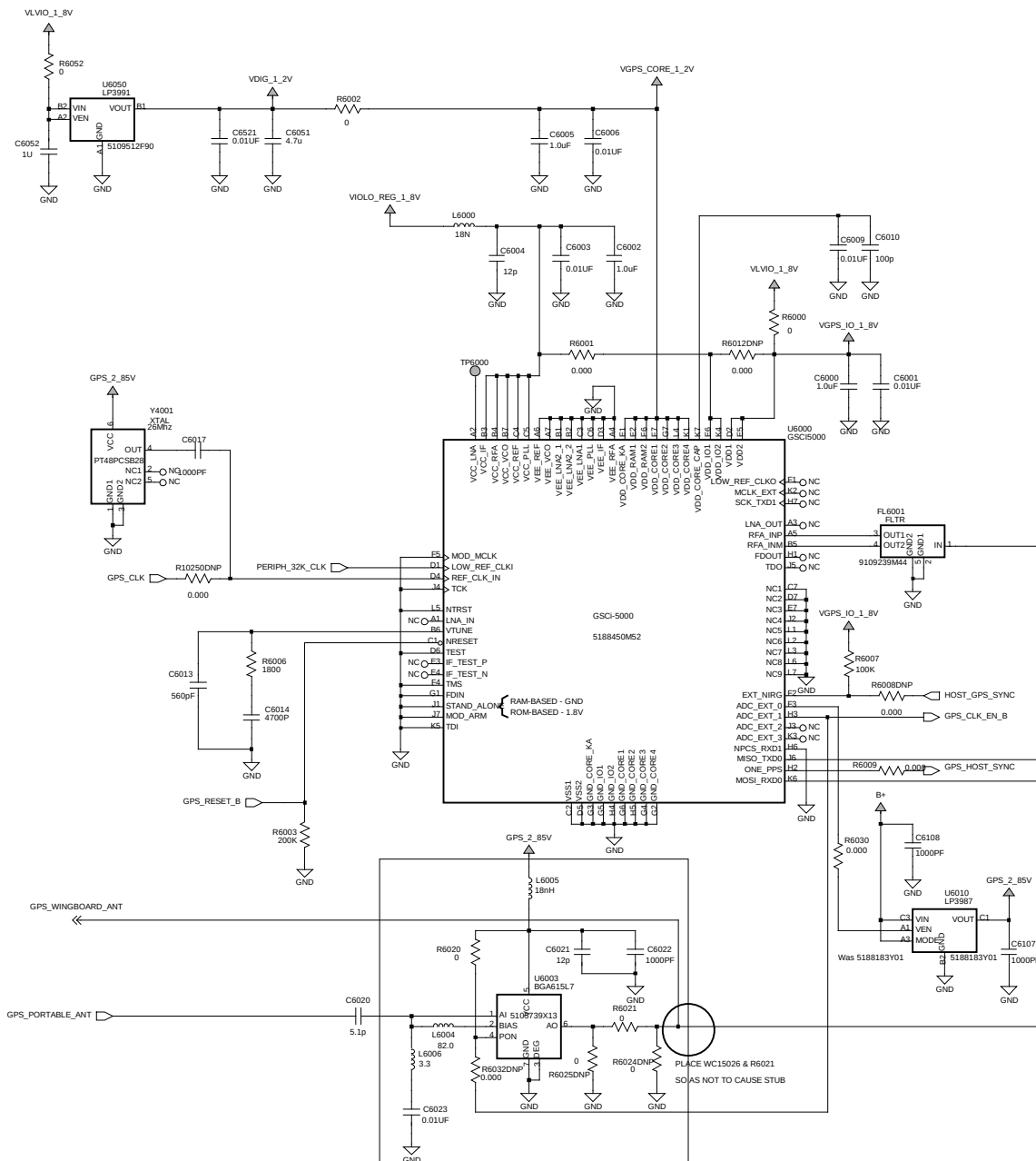
GAM 1.5 GPS Receiver
