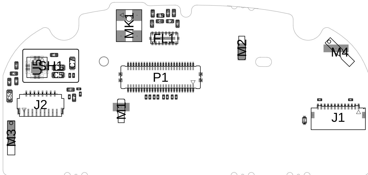
Somerset - Slider PCB - 84001378001_P1.2 - Bottom
