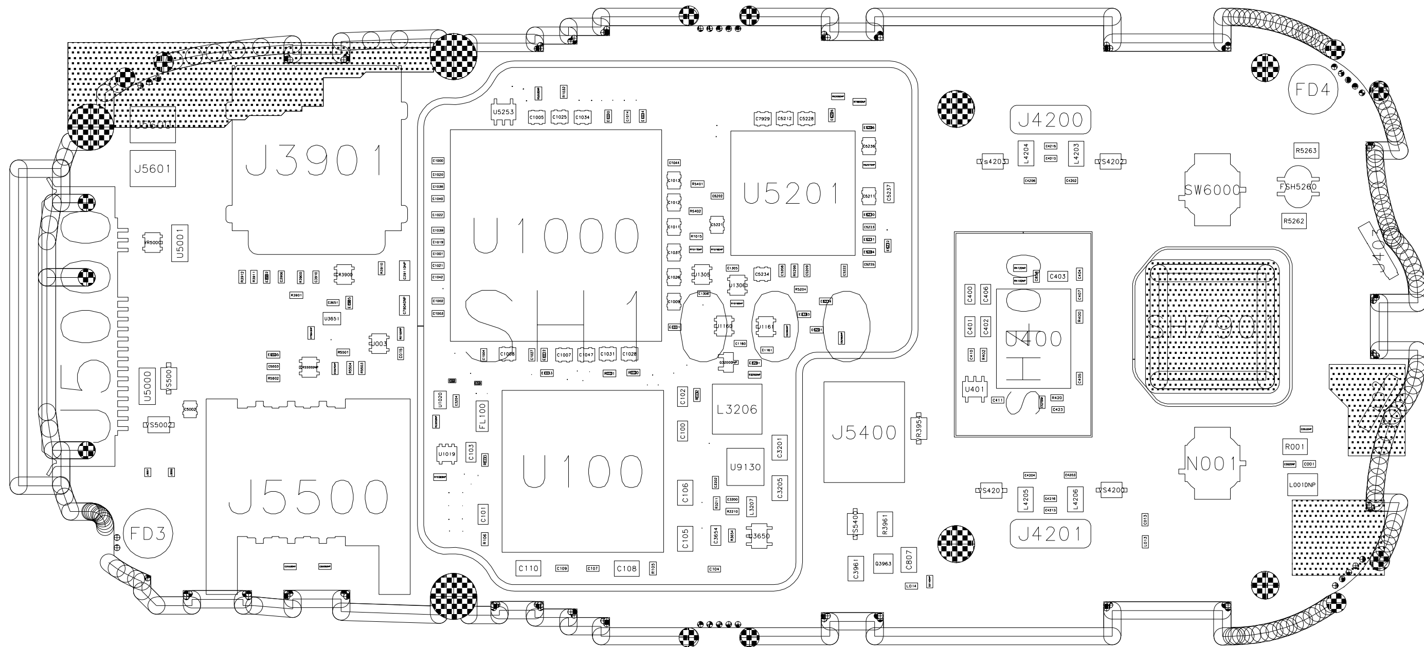
BOTTOM SIDE PARTS
