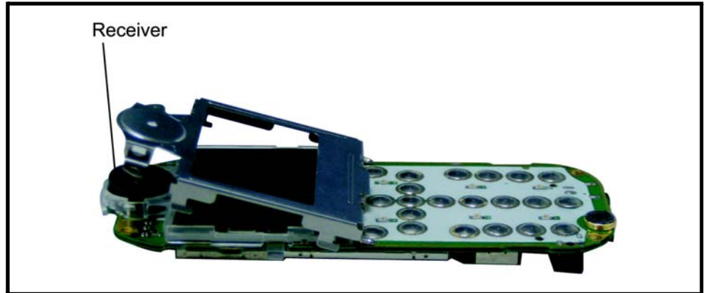
Figure 17. Pop out the receiver
