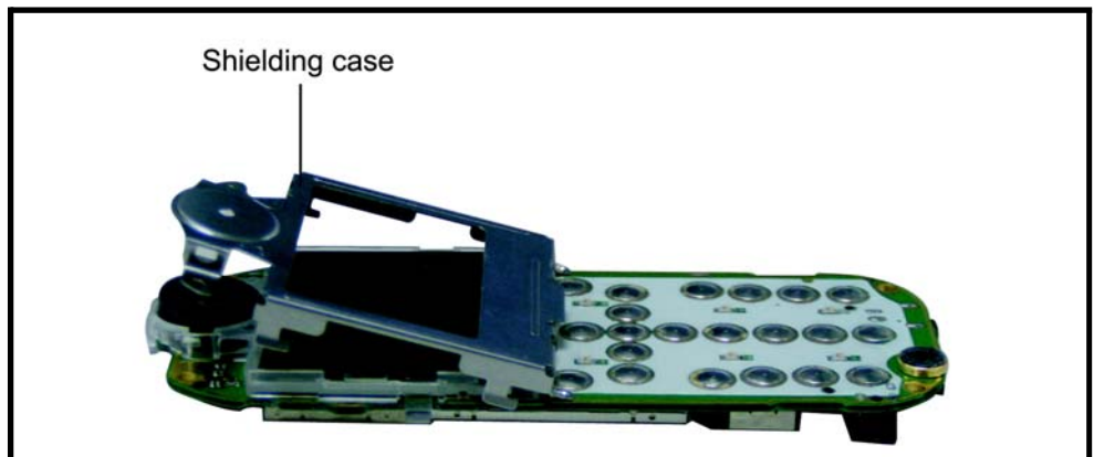
Figure 16. Pry the LCD shielding case away
