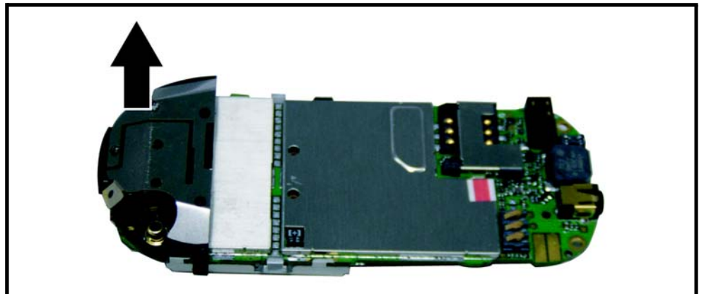
Figure 14. Gently pry off the antenna module from the Transceiver board
