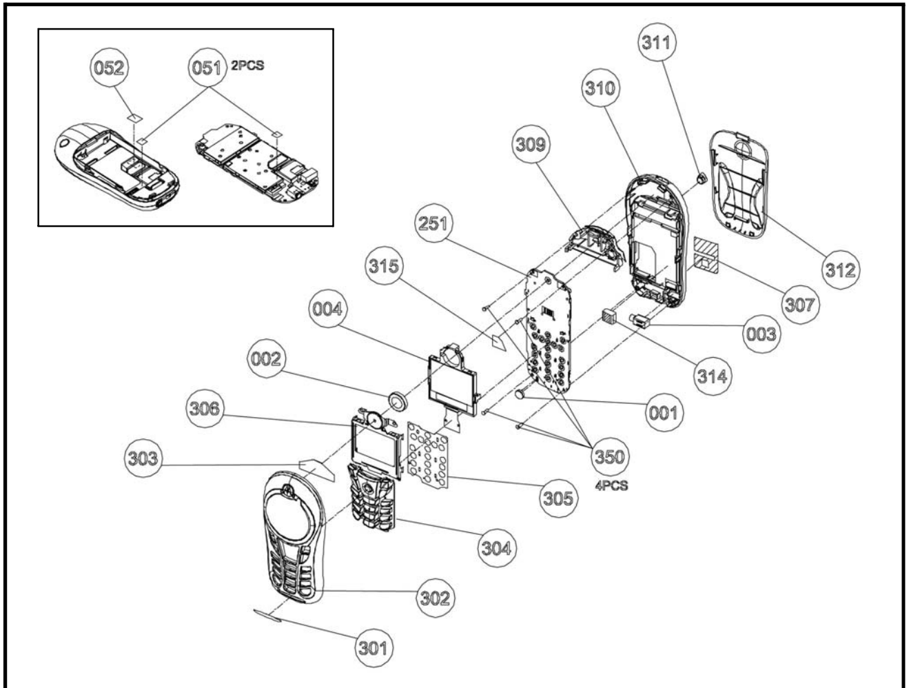
Figure 19. C115 Exploded View Diagram
