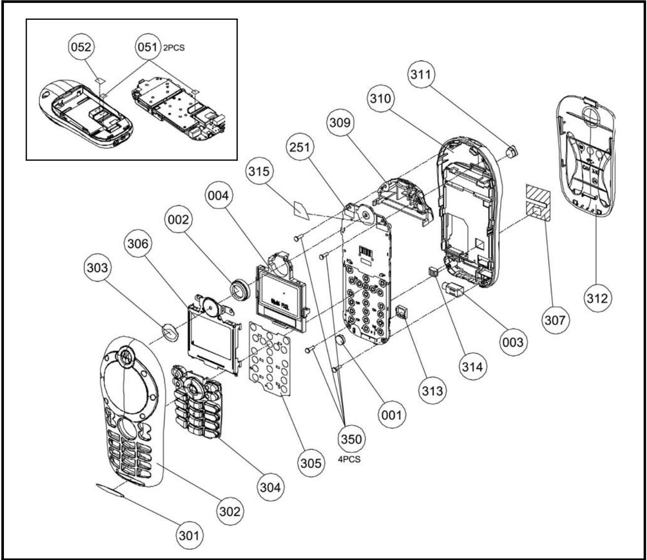
Figure 20. C116 Exploded View Diagram
