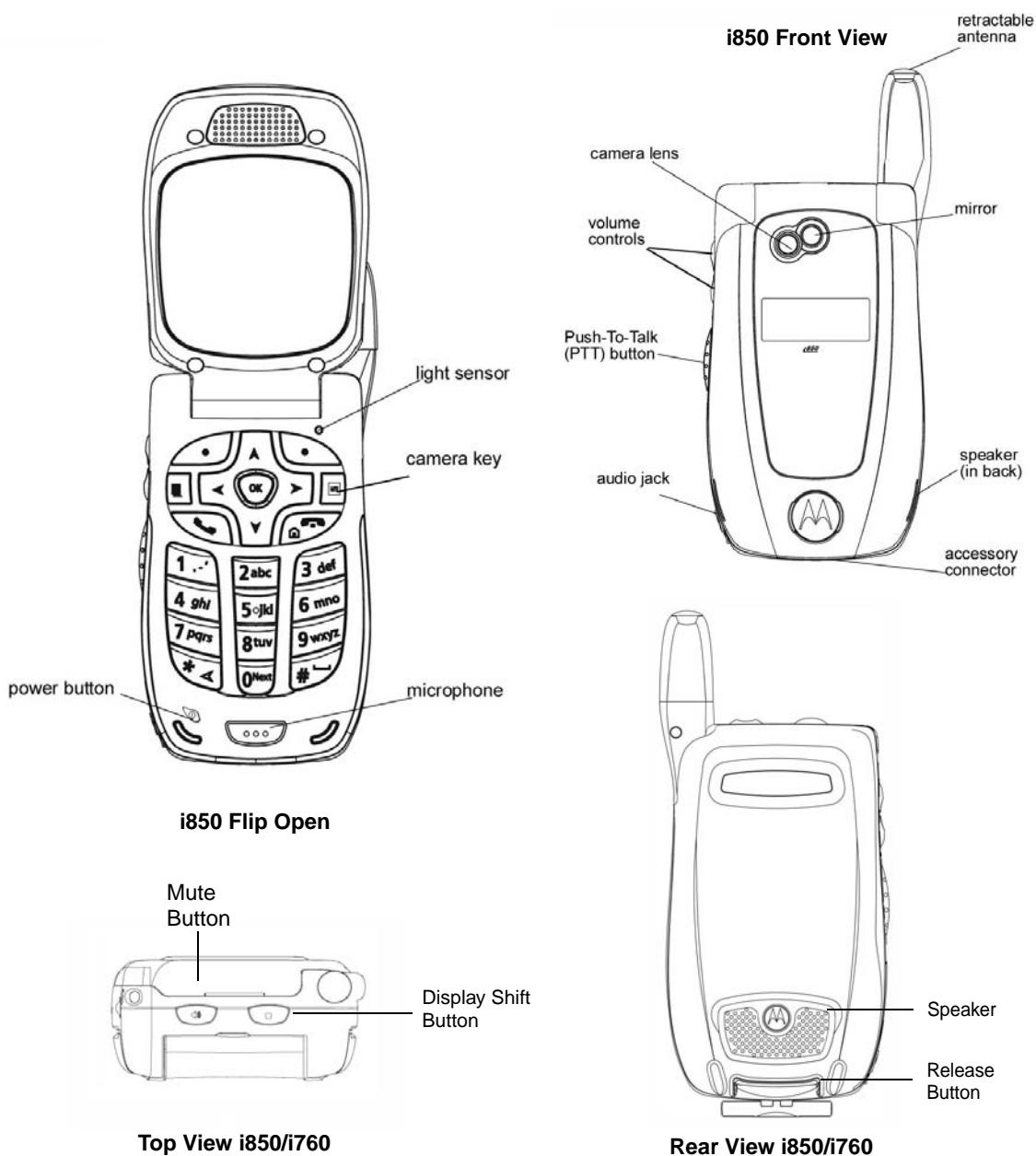
Figure 2-1. i850 Feature Views
