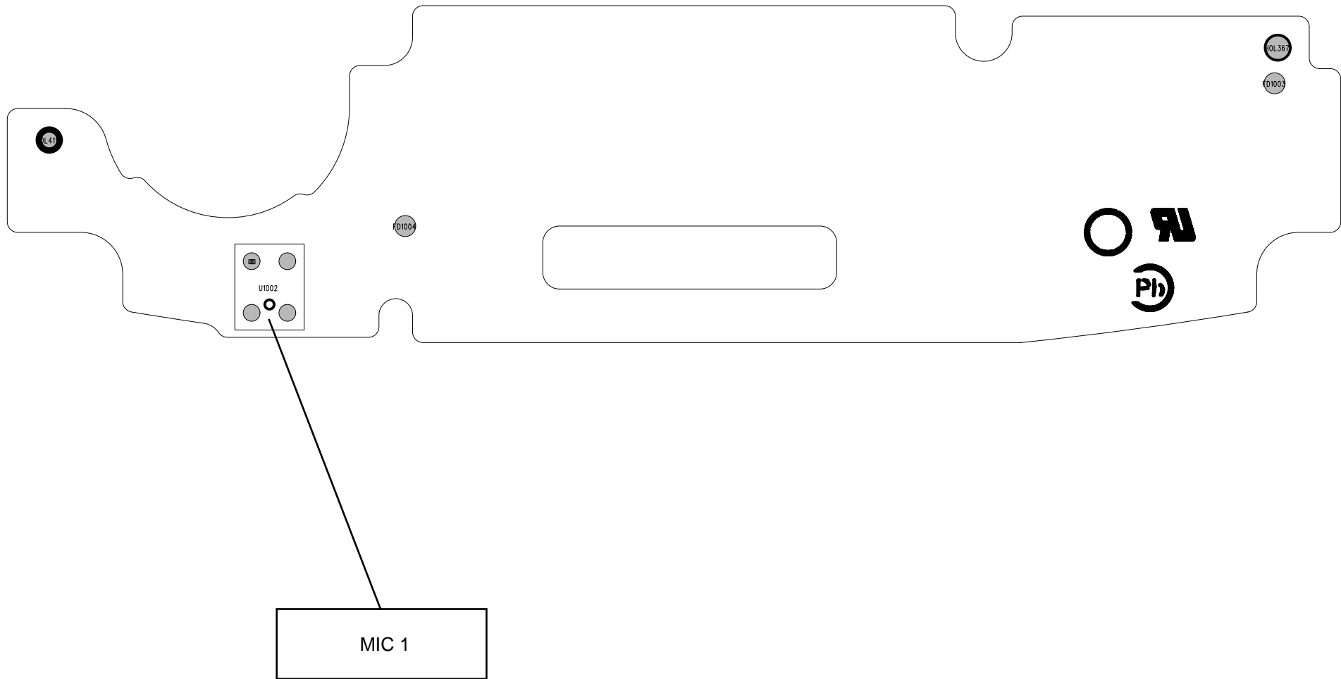
Lacrosse Sub_Board ---- TOP ----
