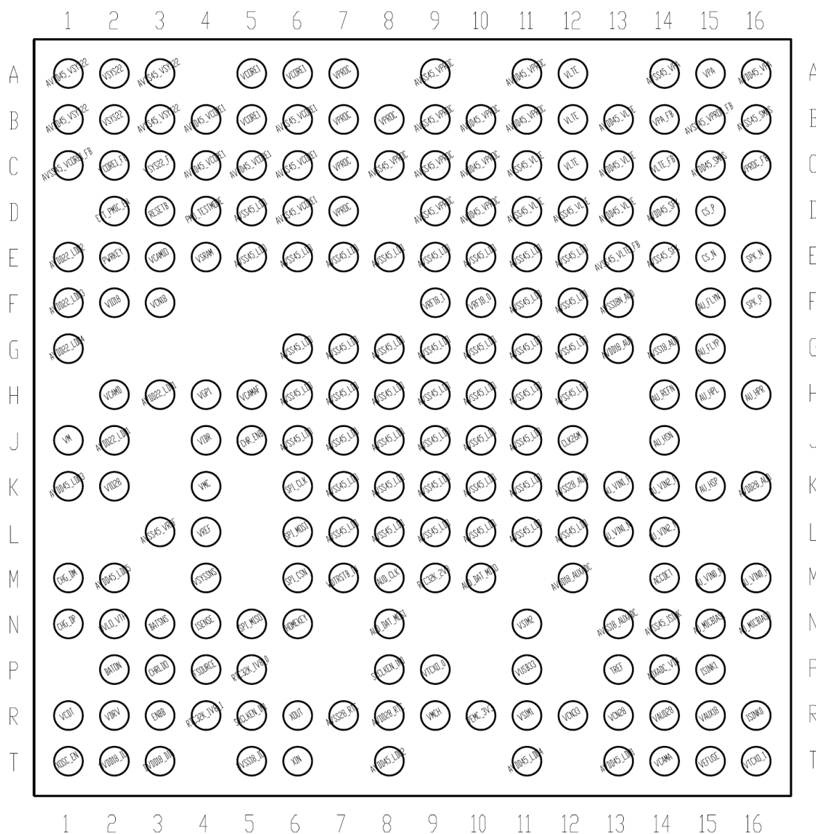
Figure 1-1. MT6328 VFBGA 206 (6.6x6.6mm) pin assignment
