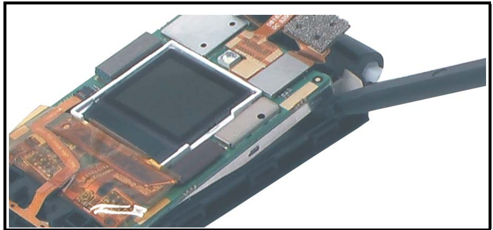
Figure 20. Removing the Display Assembly
