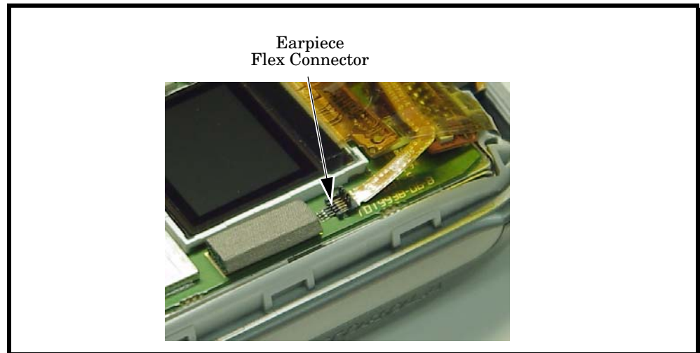
Figure 21. Disconnect the Earpiece Flex
