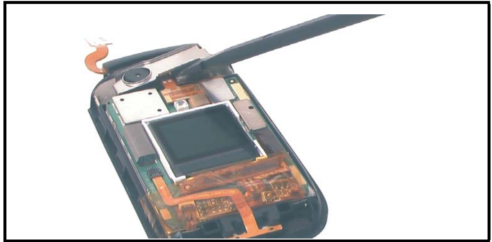
Figure 19. Removing the Imager Bracket
