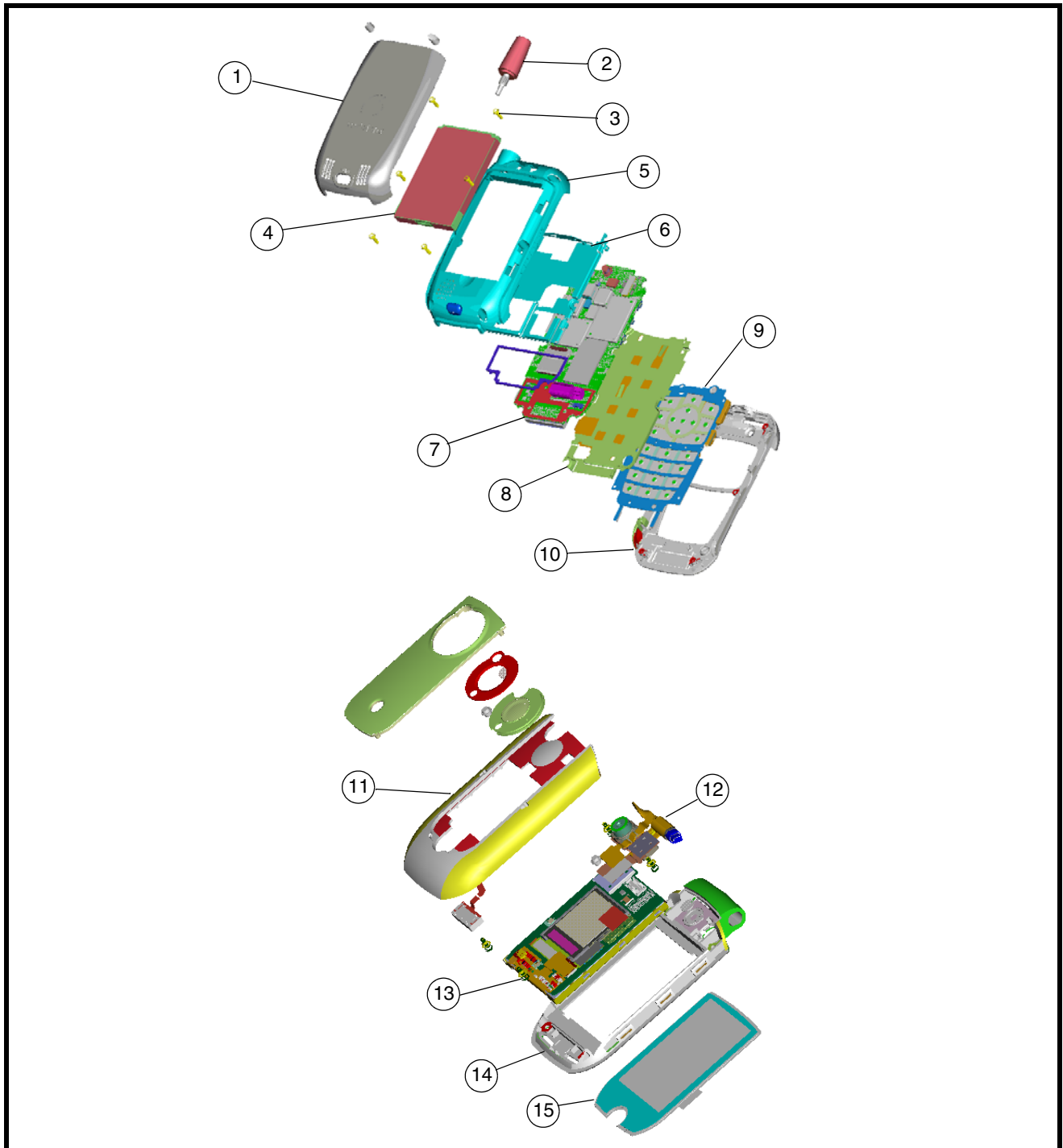
Figure 24. Exploded View Diagram
