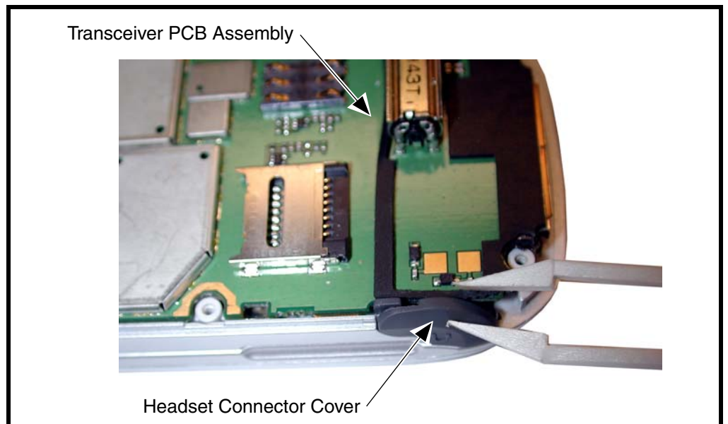
Figure 10. Removing the Headset Connector Cover
