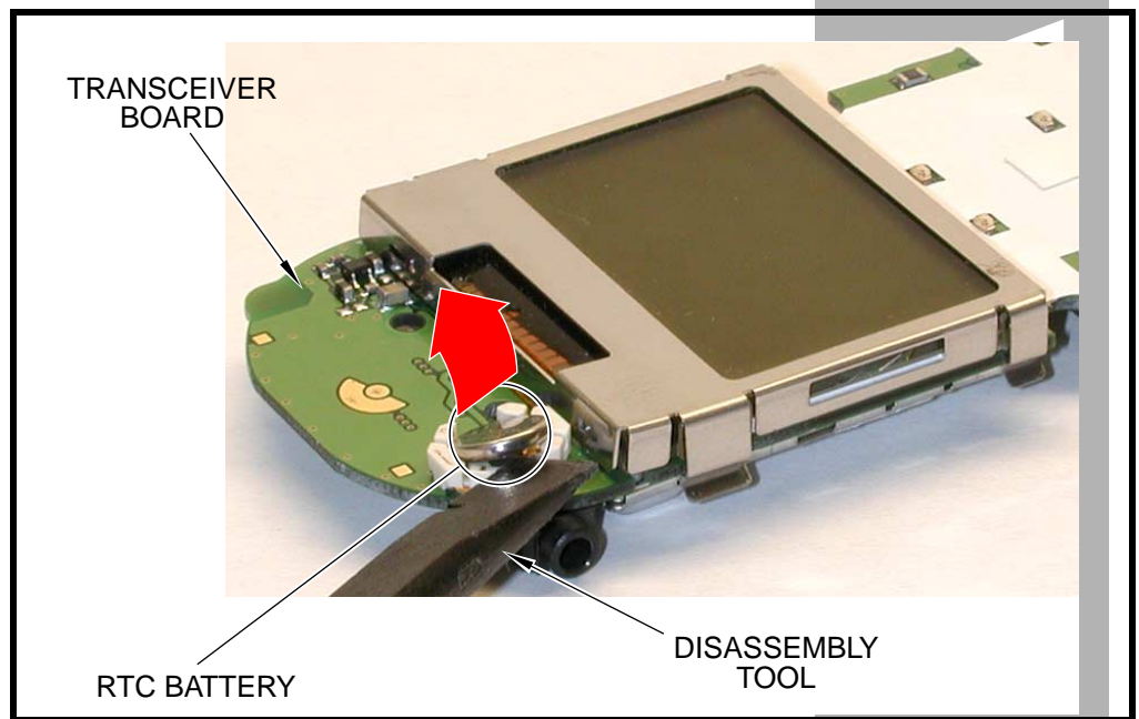
Figure 15. Removing the RTC battery
