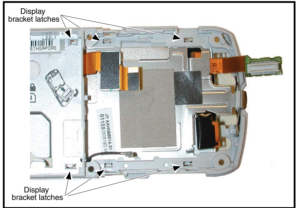
Figure 19. Removing the Display Module Latches
