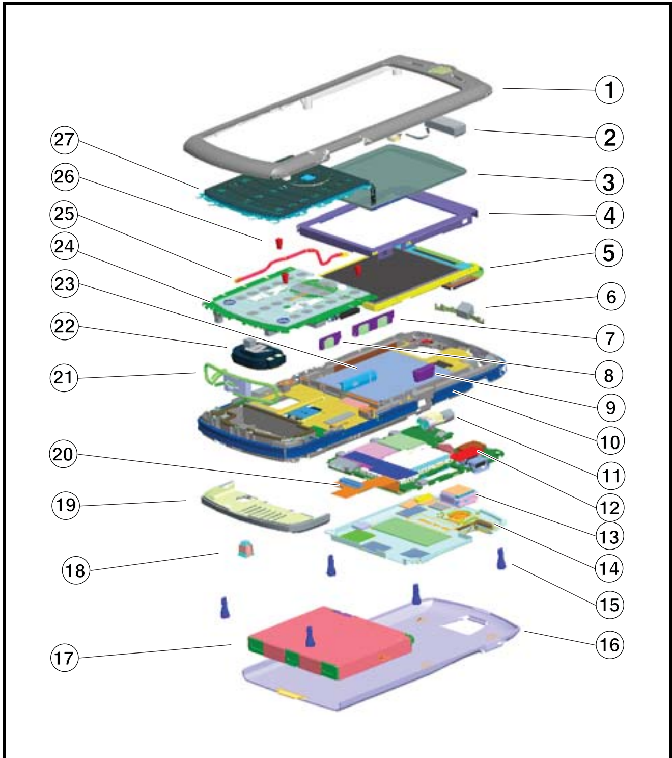
Figure 23. Exploded View Diagram
