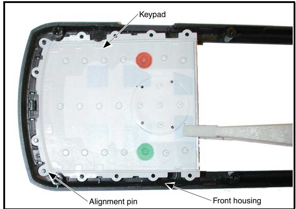
Figure 15. Removing and Replacing the Keypad
