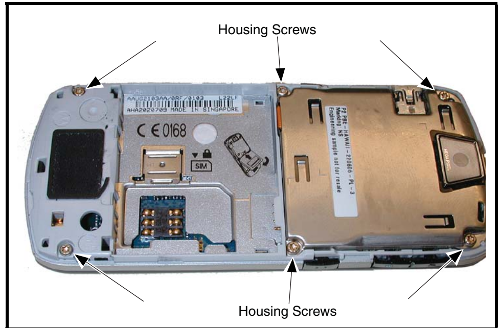
Figure 7. Removing and Replacing the Rear Housing Screws.
