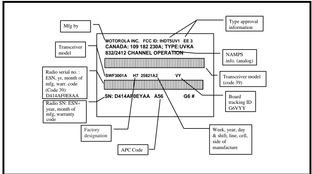
Figure 25. Telephone Identification Label
