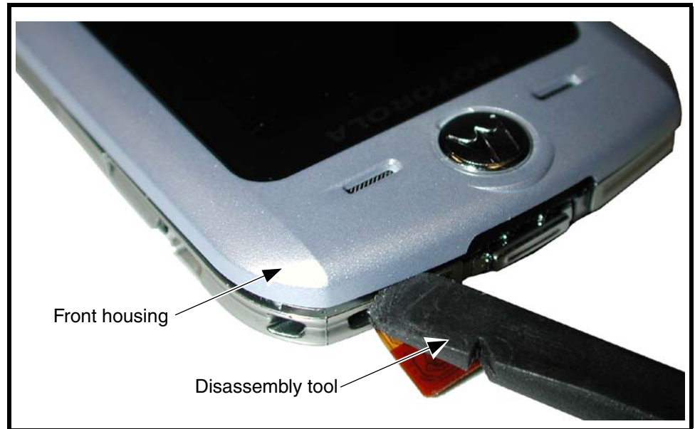
Figure 17. Releasing the Front Housing Catches
