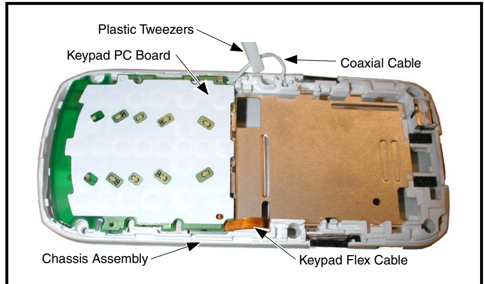
Figure 20. Removing and Replacing the Keypad PC Board
