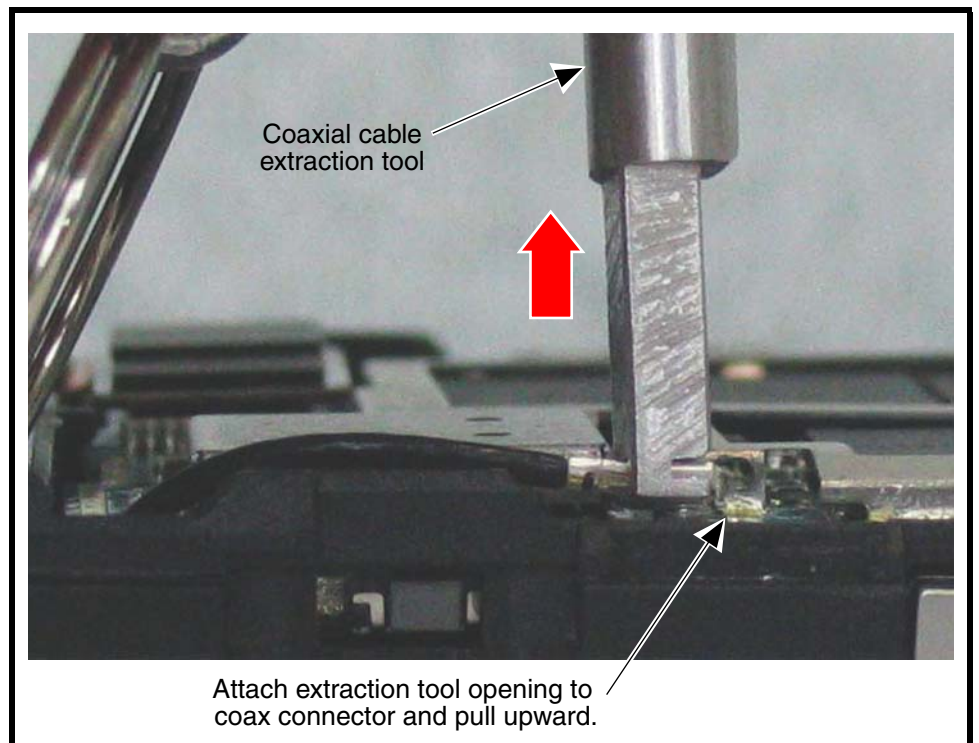
Figure 14. Coaxial Cable Extraction
