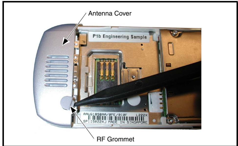
Figure 7. Removing and Replacing the RF Grommet
