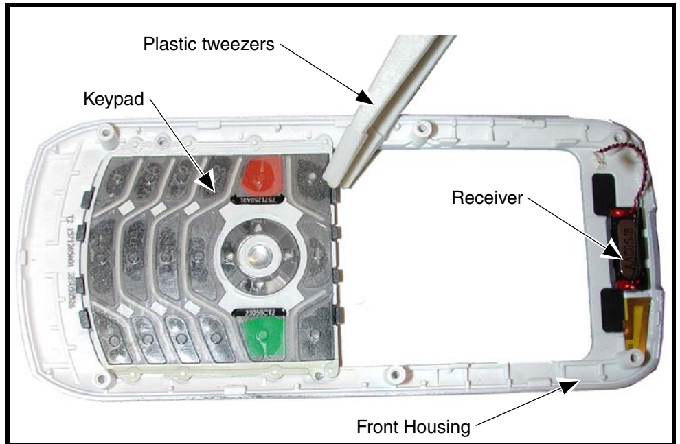
Figure 21. Removing and Replacing the Keypad
