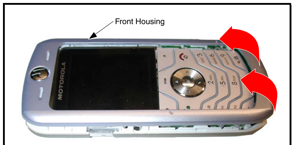
Figure 18. Removing the Front Housing
