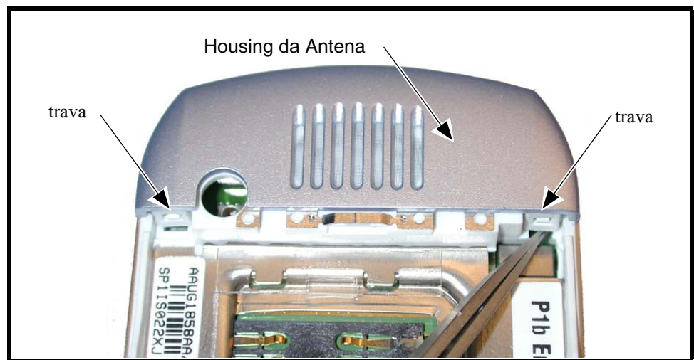
Figure 8. Removing and Replacing the Antenna Cover
