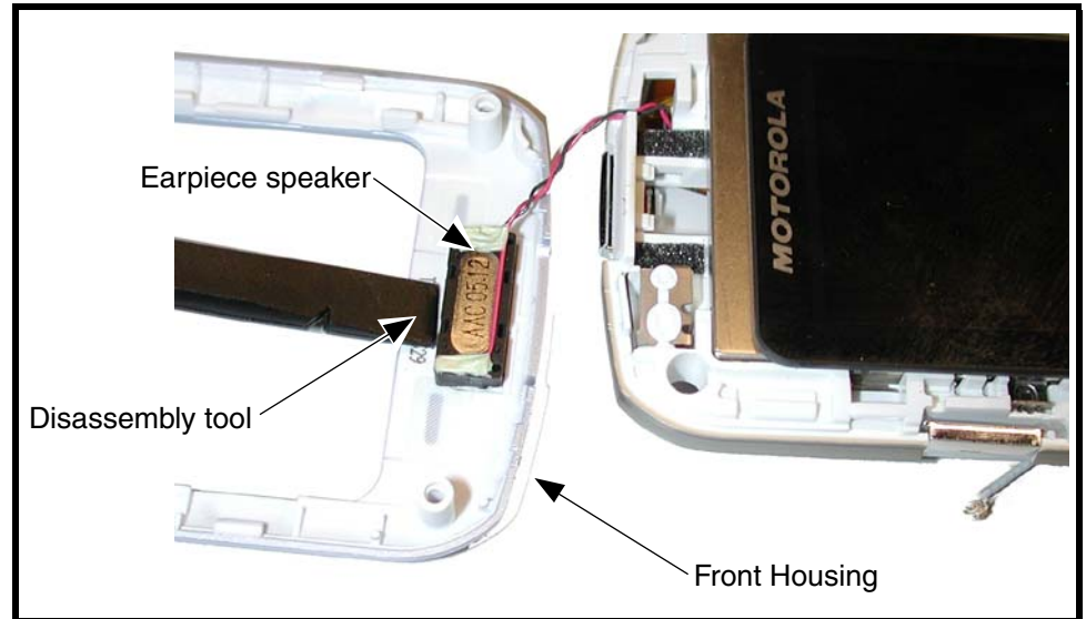
Figure 19. Removing the Earpiece Speaker from the Front Housing
