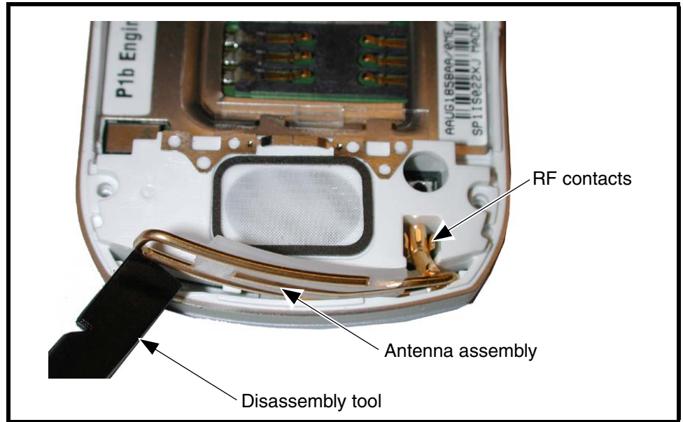
Figure 9. Removing and Replacing the Antenna
