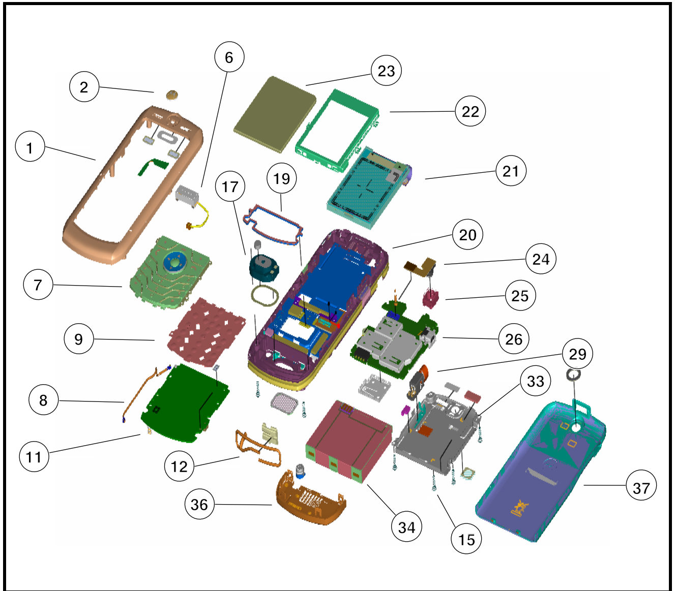
Figure 26. Exploded View Diagram
