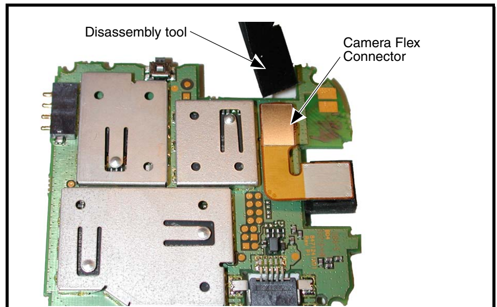
Figure 16. Removing the Camera Assembly
