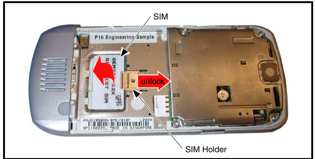
Figure 6. Removing and Replacing the SIM
