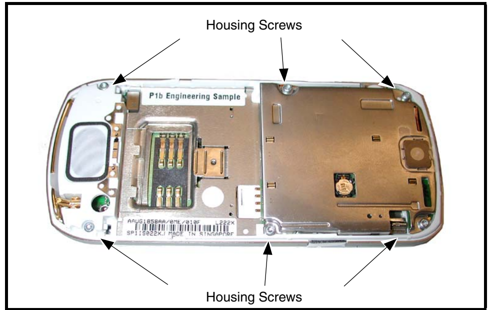
Figure 10. Removing and Replacing the Transceiver PC Board Shield.
