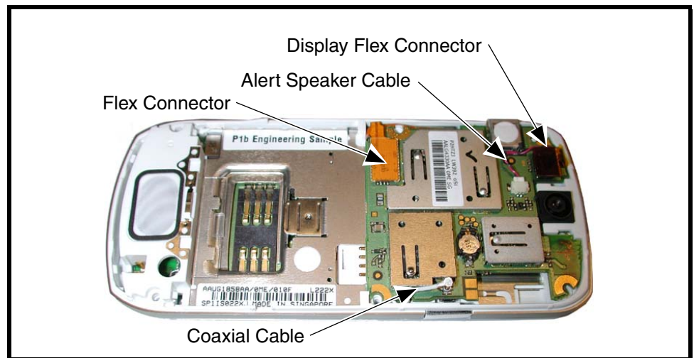
Figure 12. Removing the Transceiver PC Board Connectors
