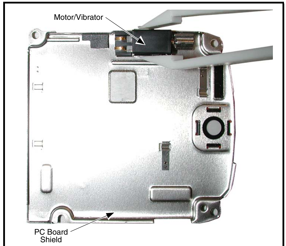
Figure 11. Removing and Replacing the Motor/Vibrator.
