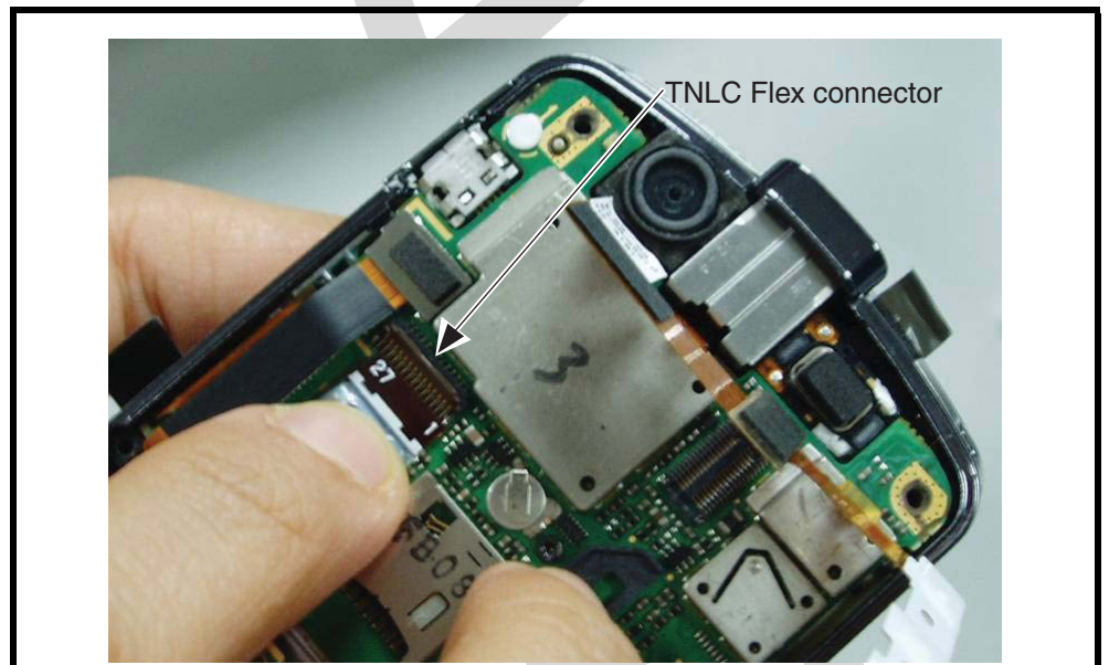
Figure 36. Connecting TNLC Flex to the Transceiver PCB
