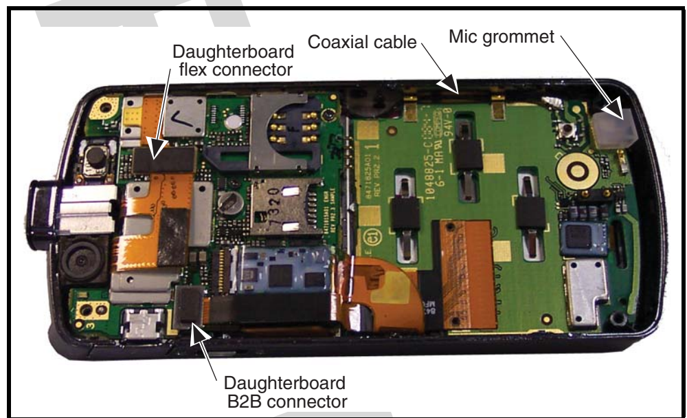
Figure 23. Removing the Transceiver Board Connectors
