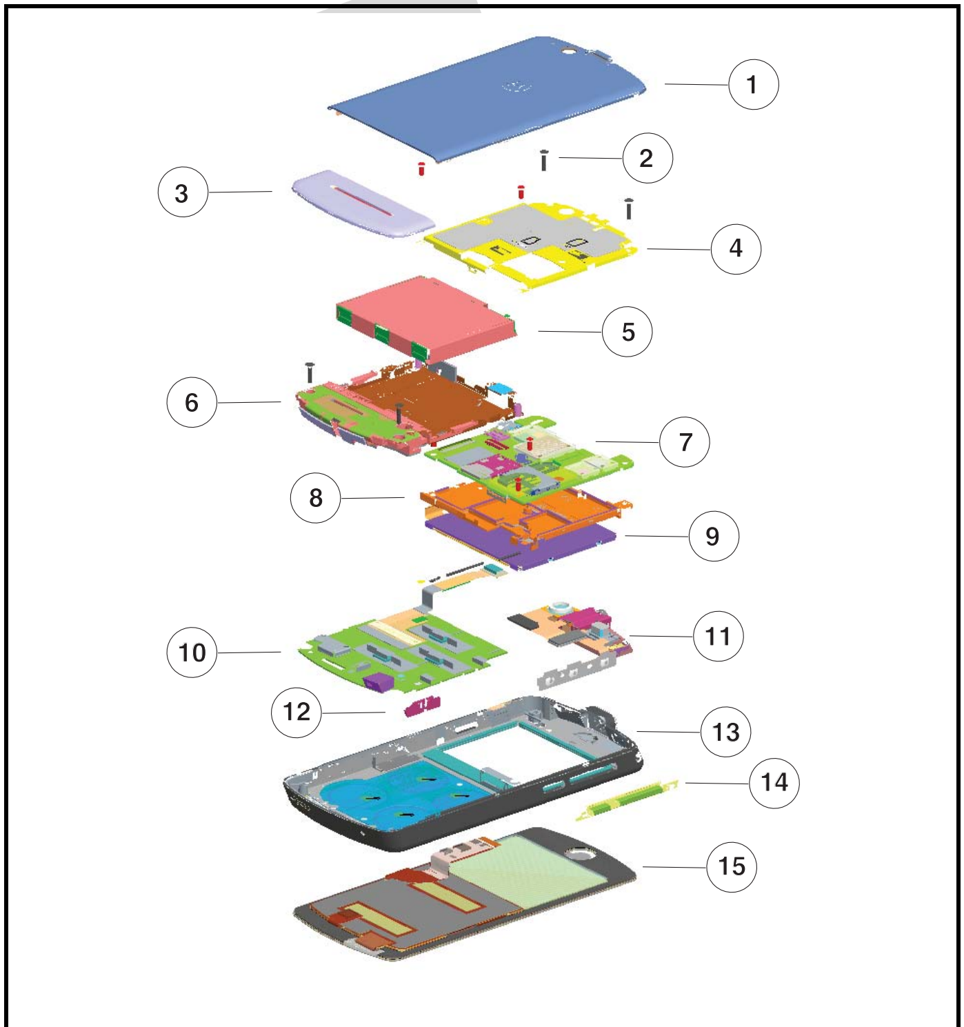
Figure 48. Exploded View Diagram
