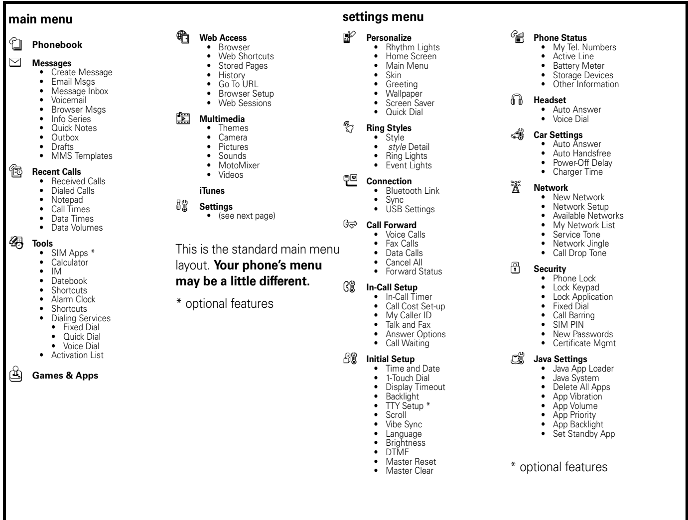
Figure 4. Menu Structure
