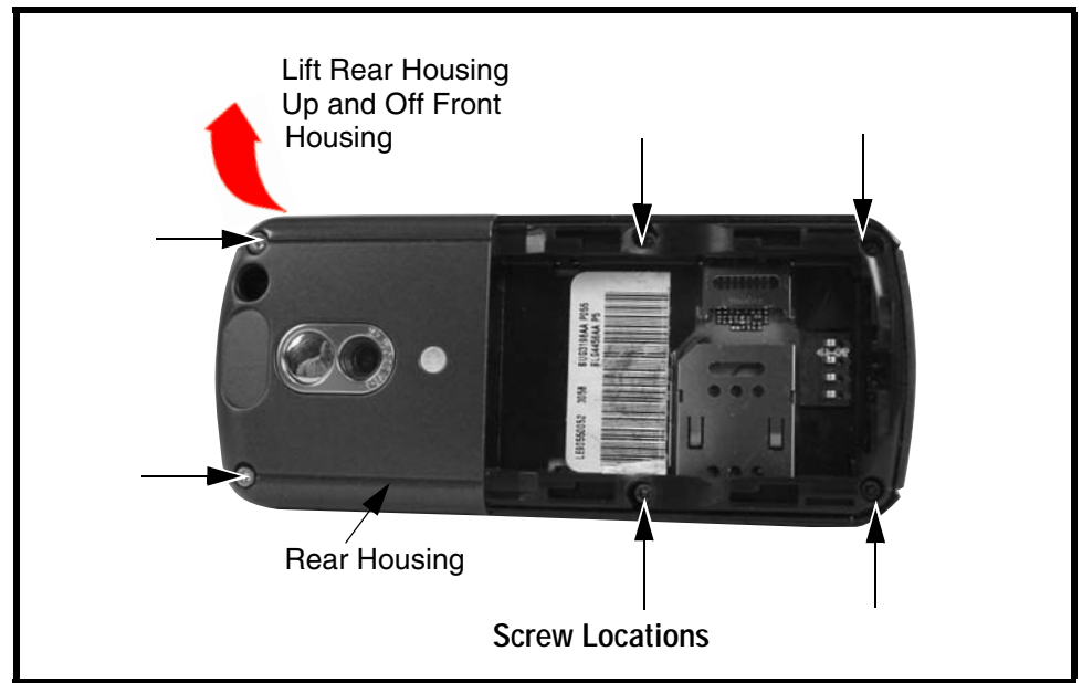
Figure 8. Removing and Replacing the Rear Housing
