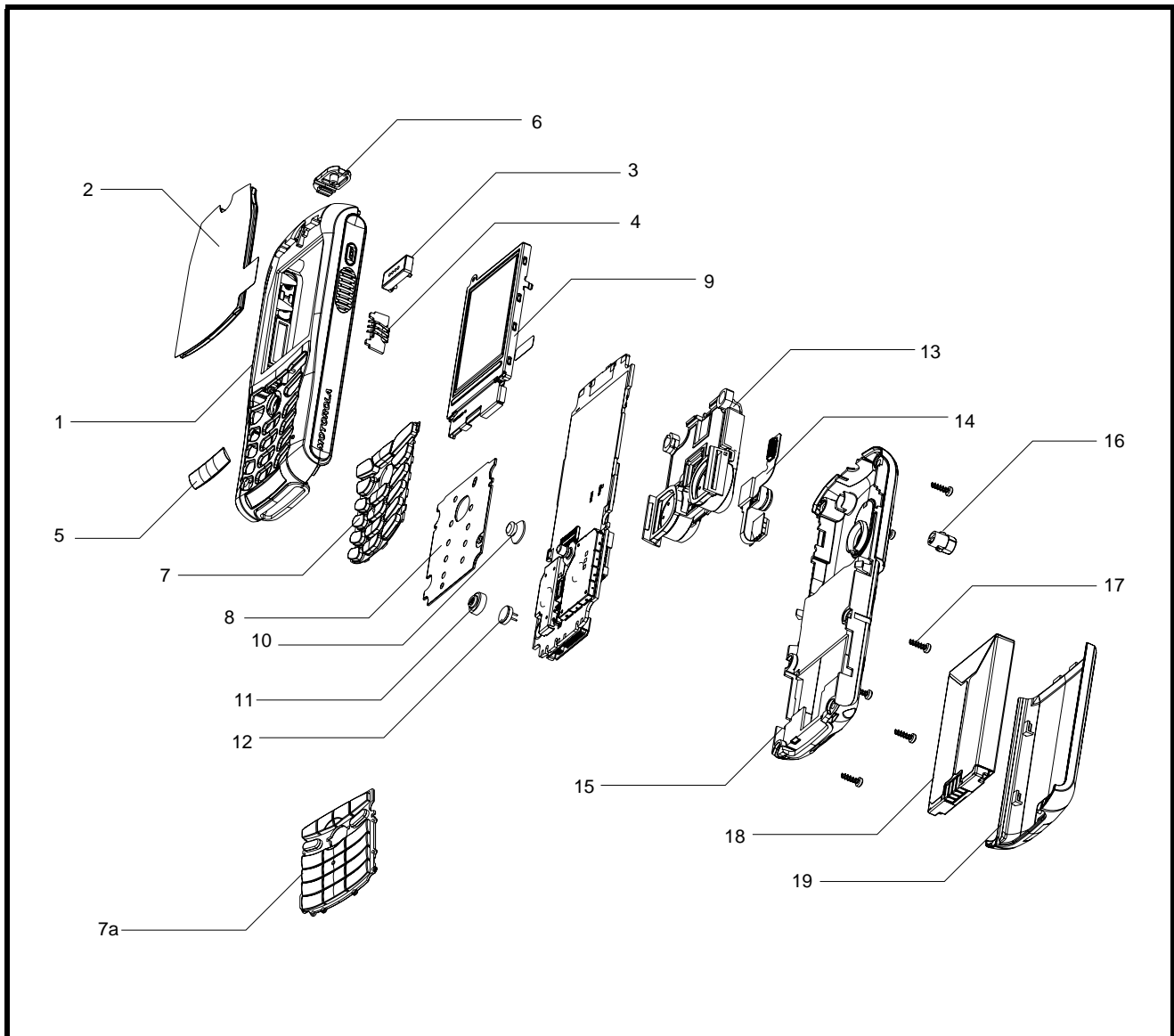
Figure 20. Exploded View Diagram
