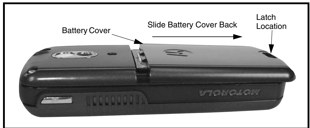
Figure 5. Removing the Battery Cover
