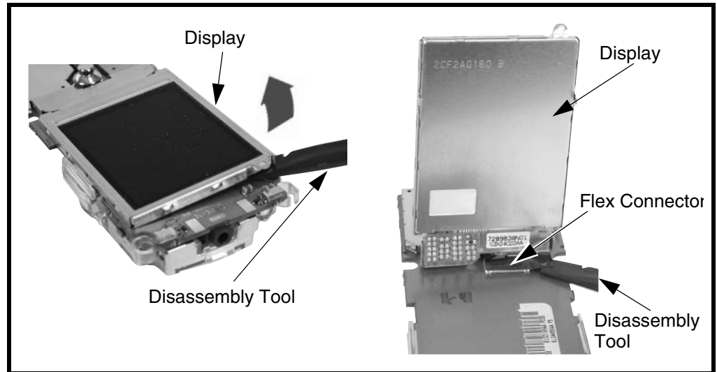
Figure 15. Removing and Replacing the Display
