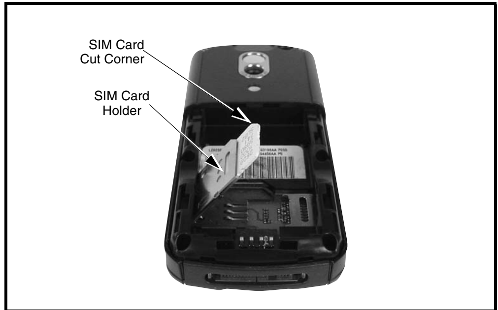
Figure 7. Removing and Replacing the SIM
