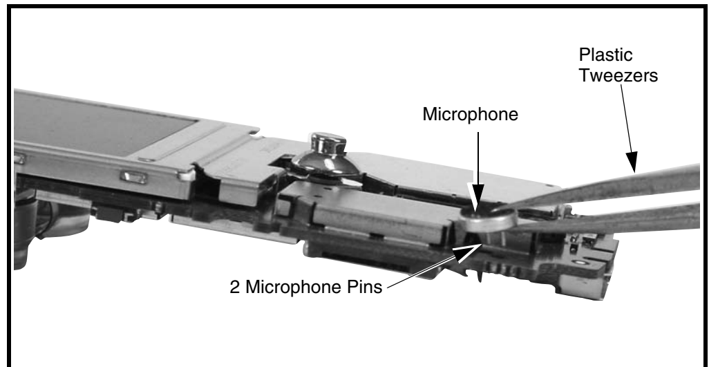
Figure 11. Removing and Replacing the Microphone
