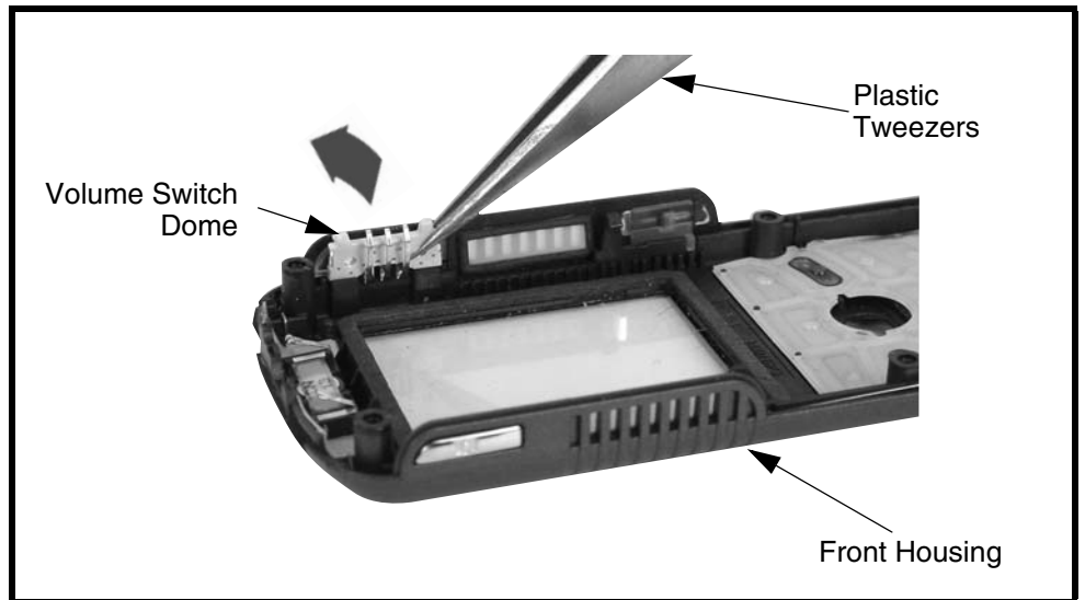
Figure 14. Removing and Replacing the Volume Switch Dome
