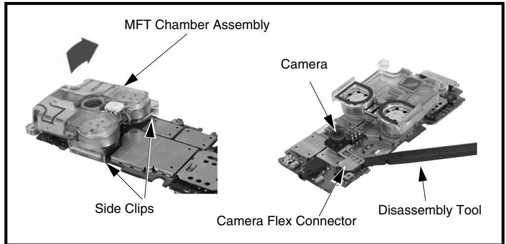
Figure 16. Removing and Replacing the MFT Chamber Assembly
