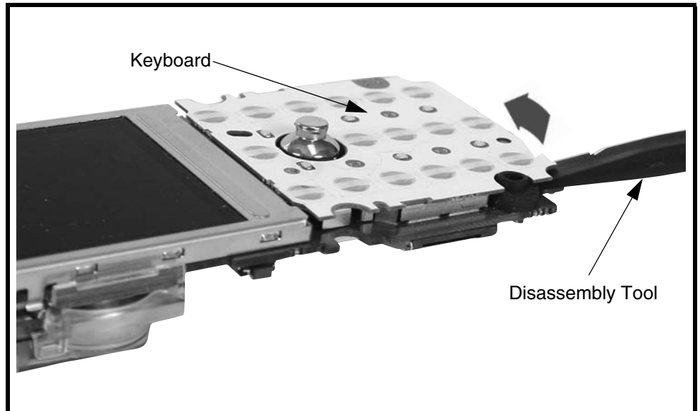
Figure 10. Removing and Replacing the Keyboard
