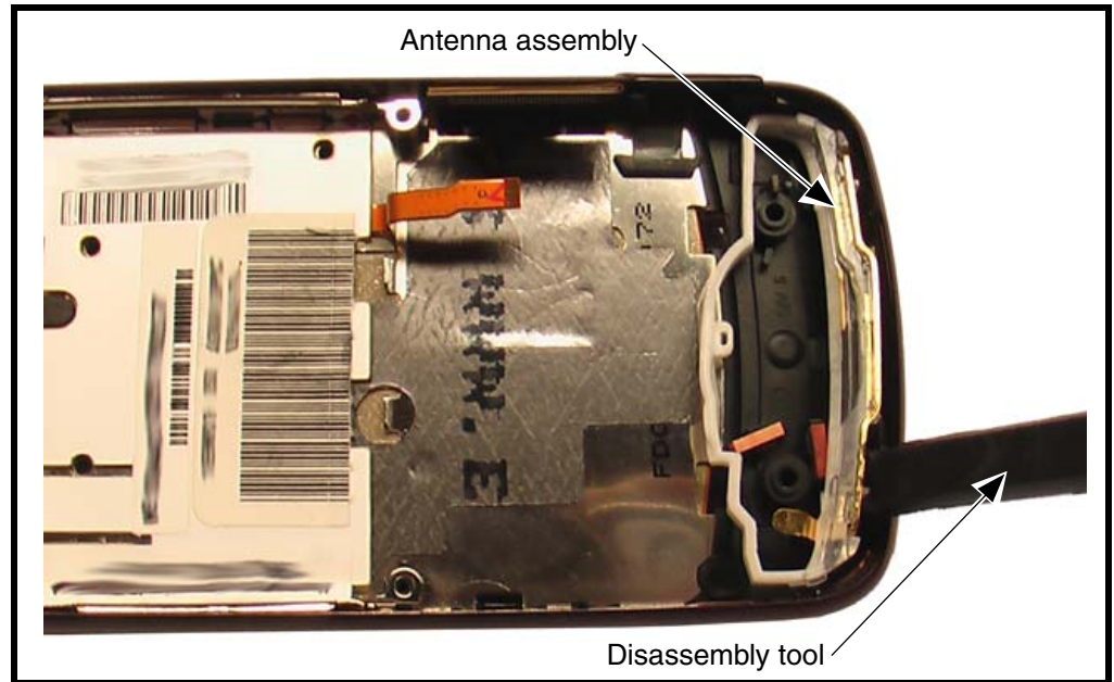
Figure 13. Removing the Antenna Assembly
