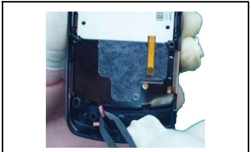
Figure 74. installing Speaker Contacts
