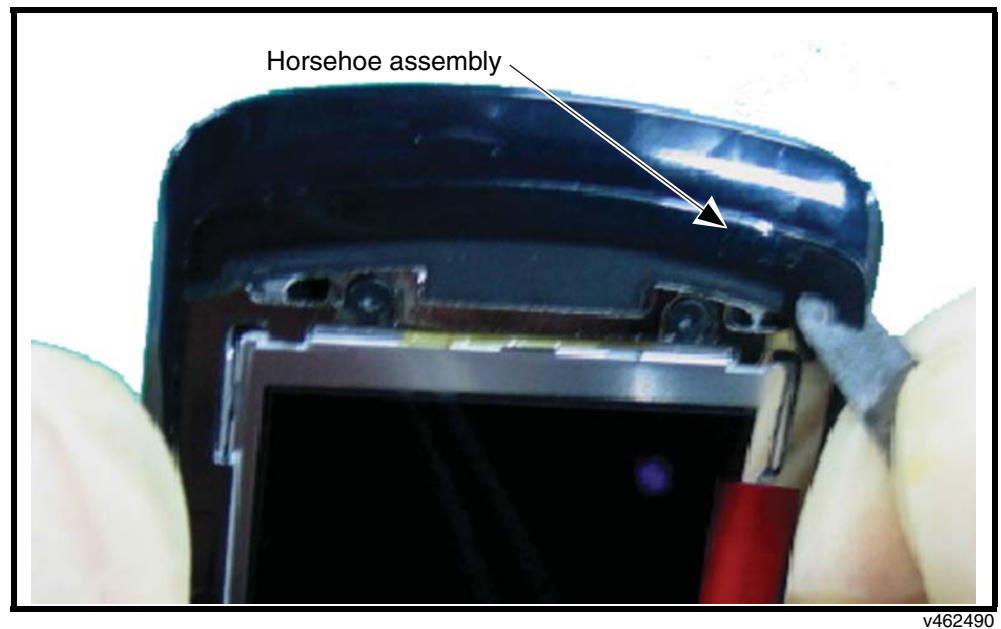
Figure 32. Removing the Horseshoe Assembly
