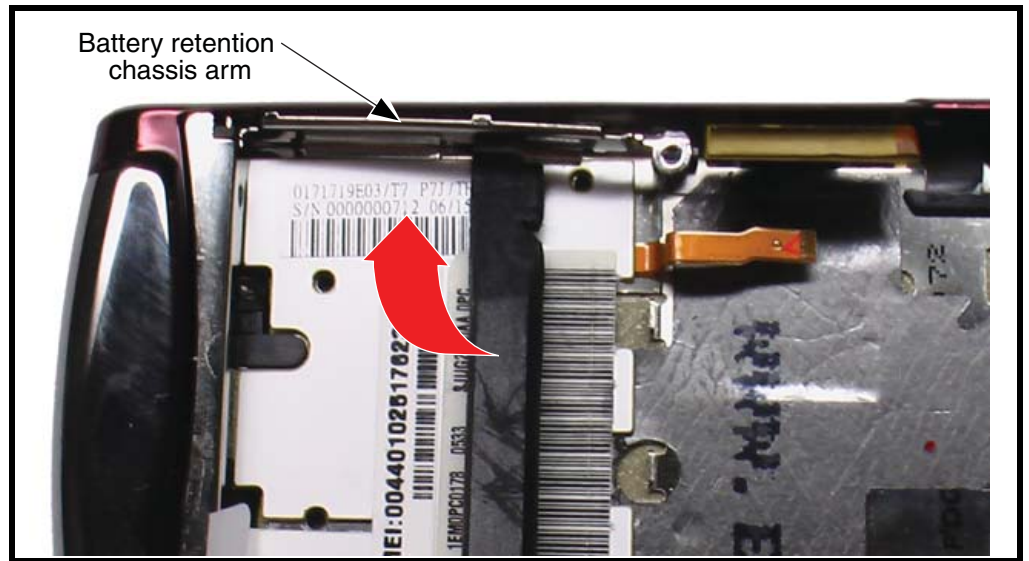
Figure 16. Removing the Battery Retention Chassis Arm
