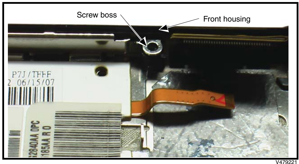
Figure 23. Installing the Battery Retention Chassis
