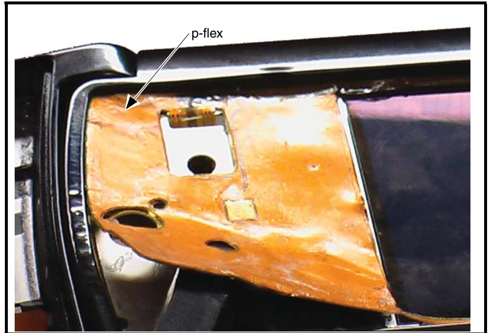
Figure 30. Removing the P-Flex
