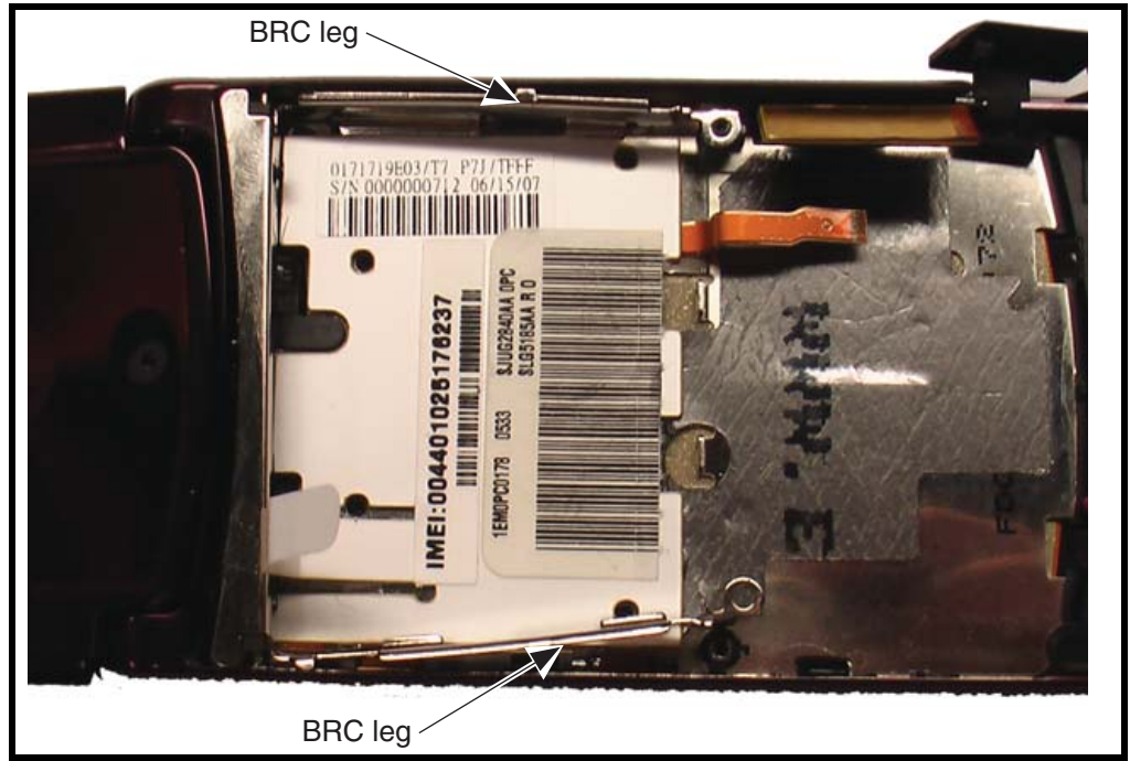
Figure 22. Installing the Battery Retention Chassis
