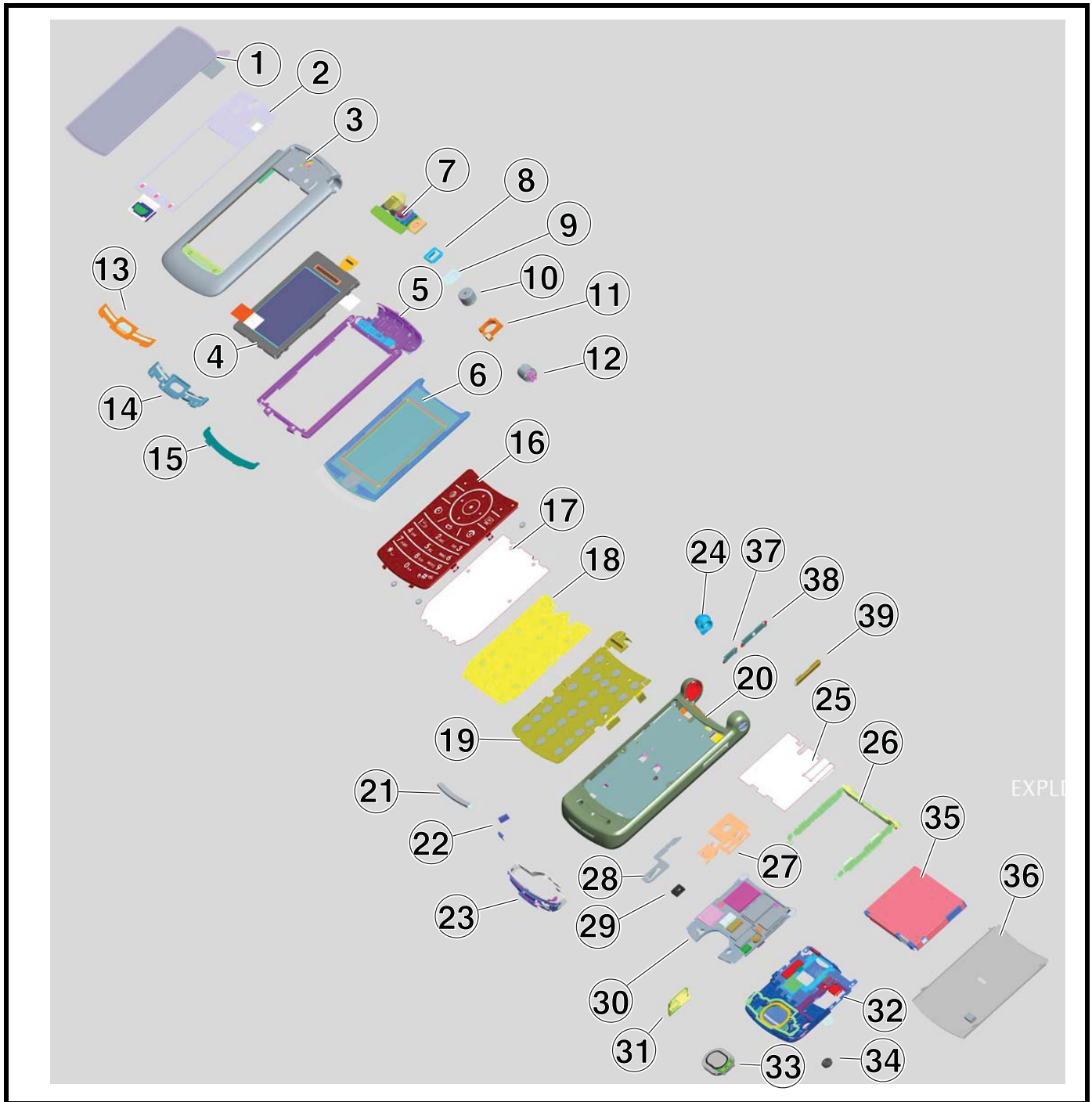
Figure 86. Exploded View Diagram
