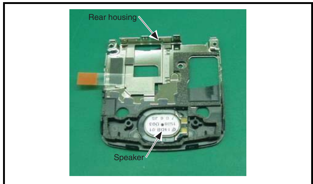
Figure 9. Replacing the Speaker
