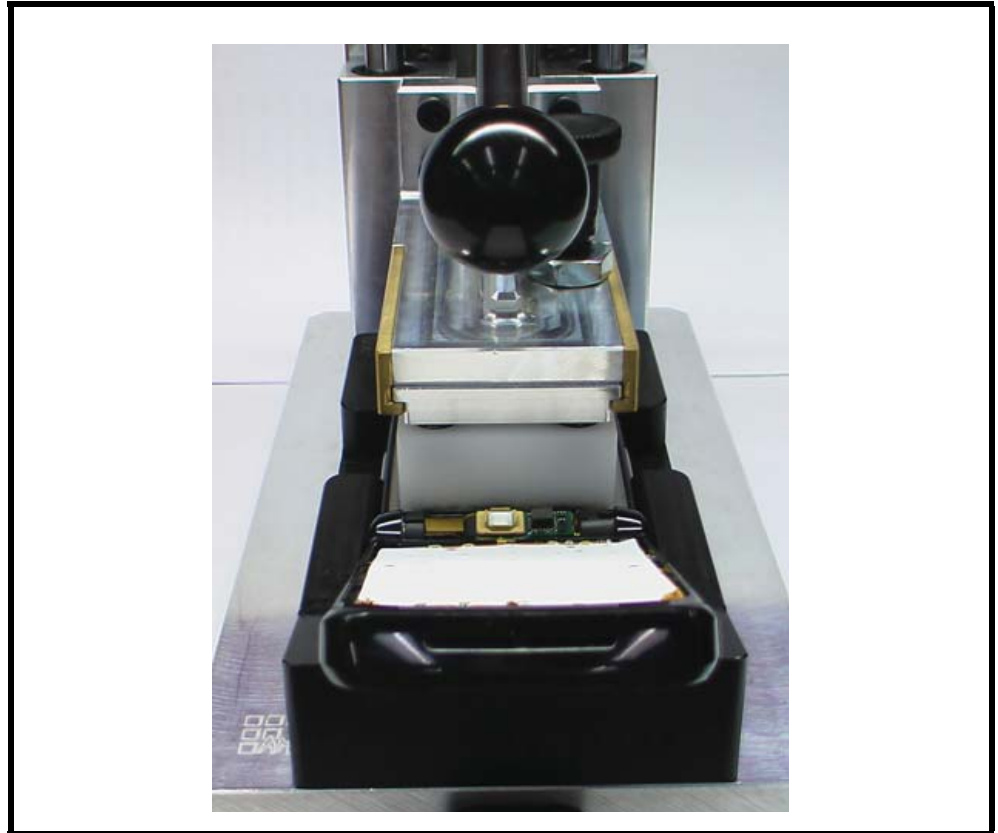
Figure 71. CLI Lens Press Fixture Closed
