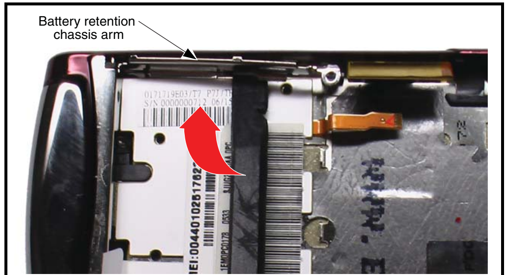
Figure 19. Removing the Battery Retention Chassis Arm
