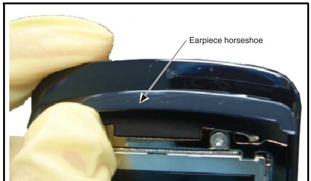
Figure 80. Installing the Earpiece Horseshoe
