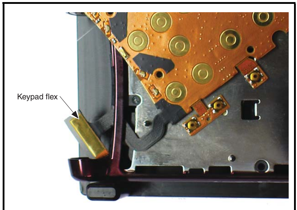
Figure 47. K-flex Connector
