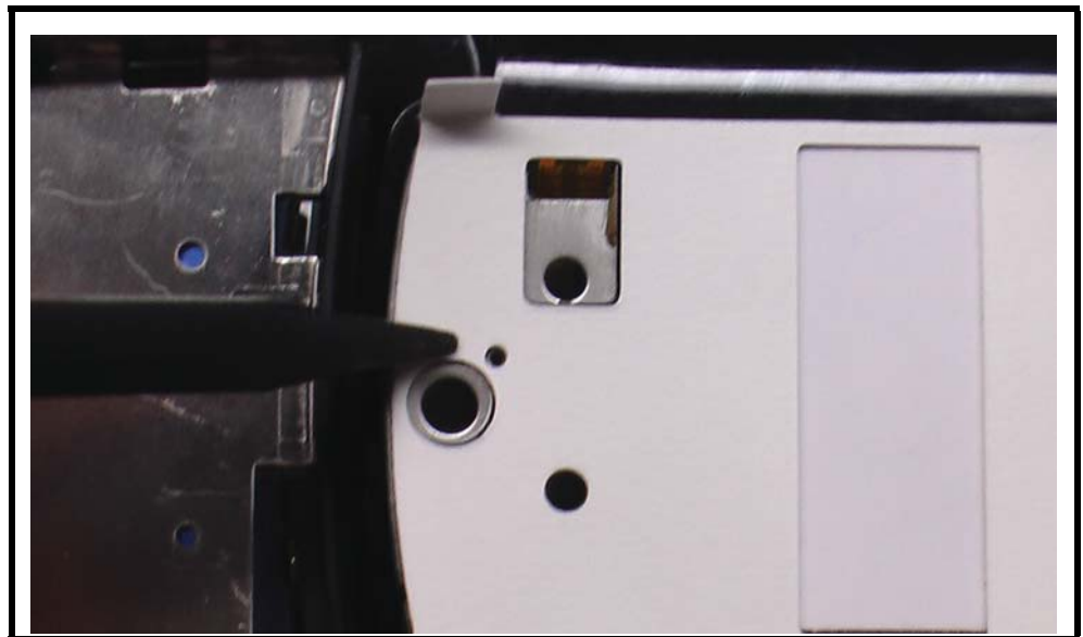
Figure 69. Attaching the P-Flex
