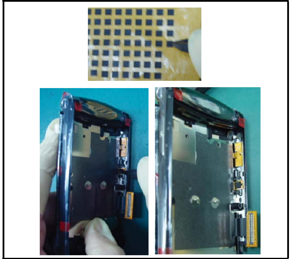
Figure 52. Installing the Smart Key Keypad Flex Pad
