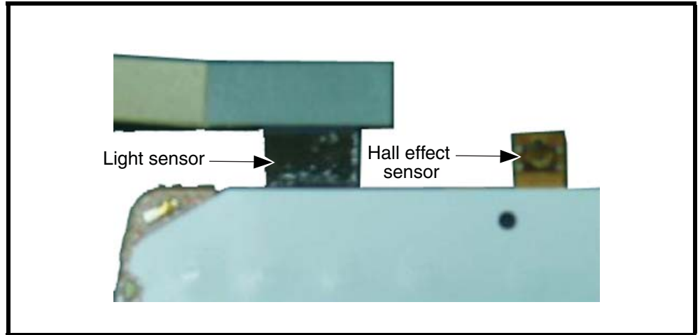
Figure 46. Protecting the K-Flex Sensors
