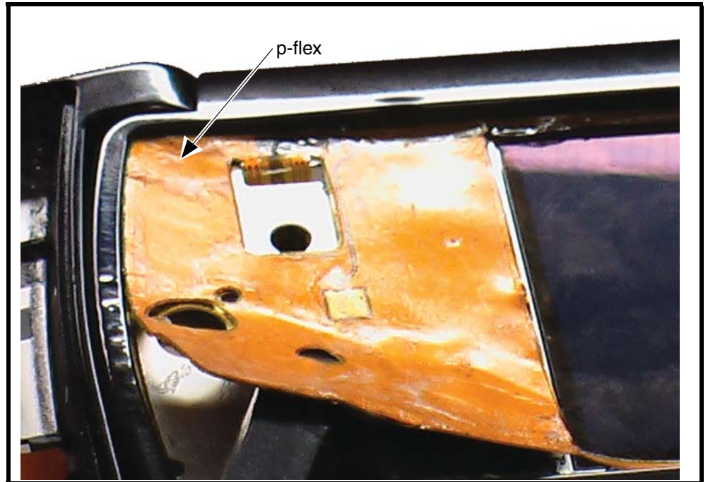
Figure 37. Removing the P-Flex
