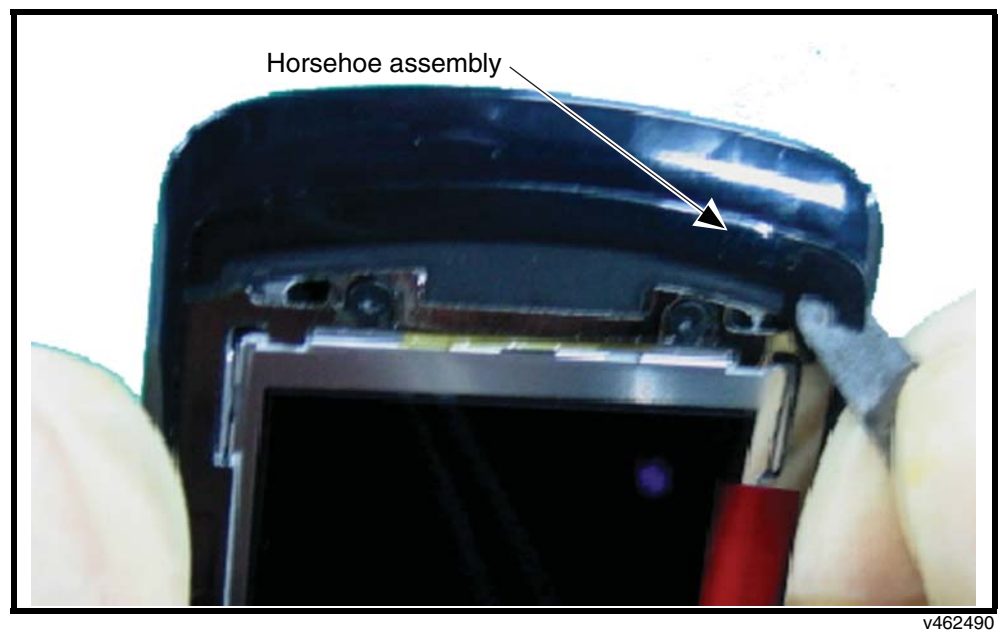
Figure 39. Removing the Horseshoe Assembly
