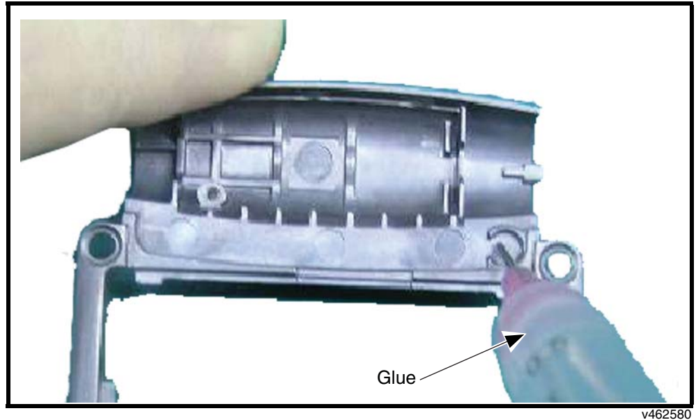
Figure 73. Installing Magnet Glue to the Flip Inner Assembly
