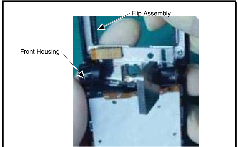
Figure 60. Installing the Flip Assembly
