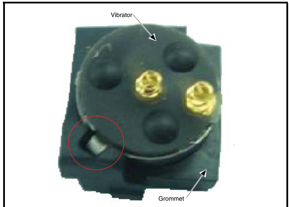
Figure 63. Installing the Vibrator Grommet
