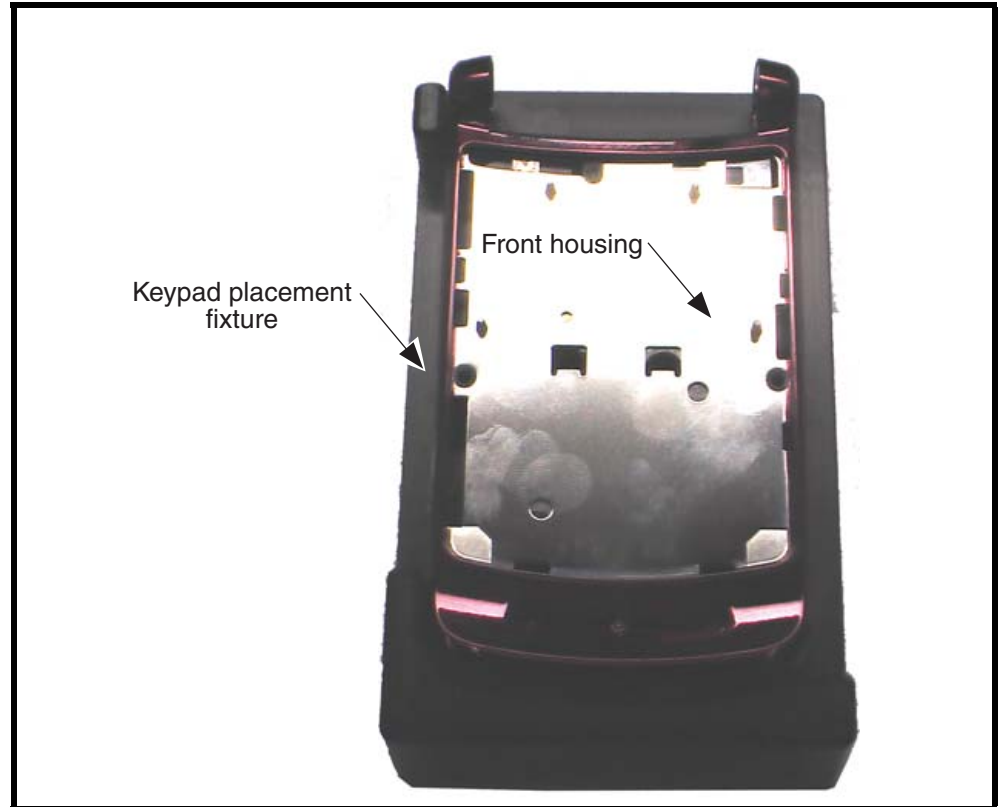
Figure 45. Keypad Placement Fixture
