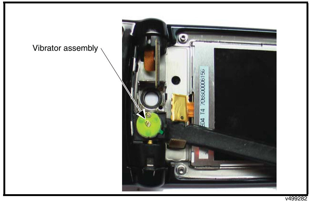
Figure 38. Removing the Vibrator Assembly
