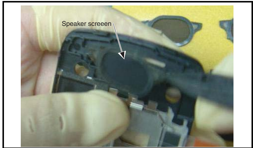
Figure 8. Replacing the Speaker Screen
