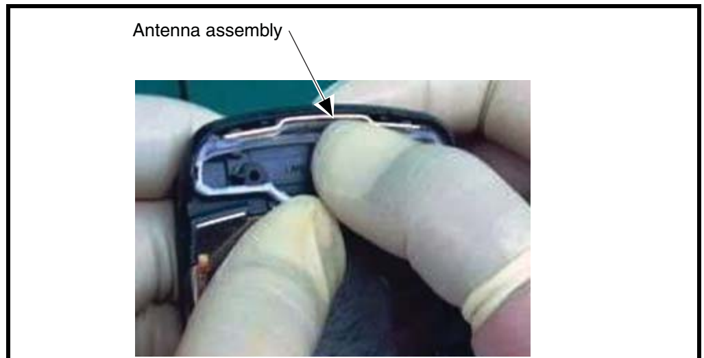
Figure 17. Installing the Antenna Assembly
