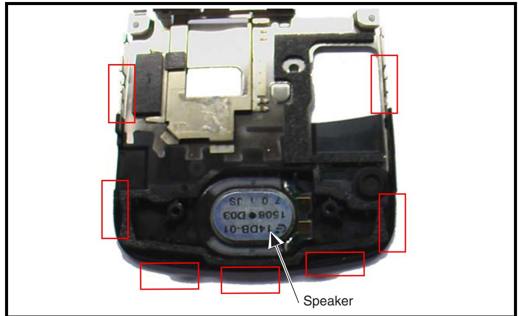
Figure 11. Rear Housing Latches
