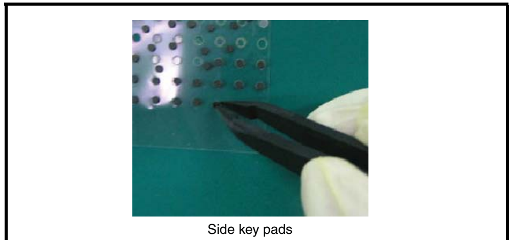
Figure 54. Peeling the Side Key Pads
