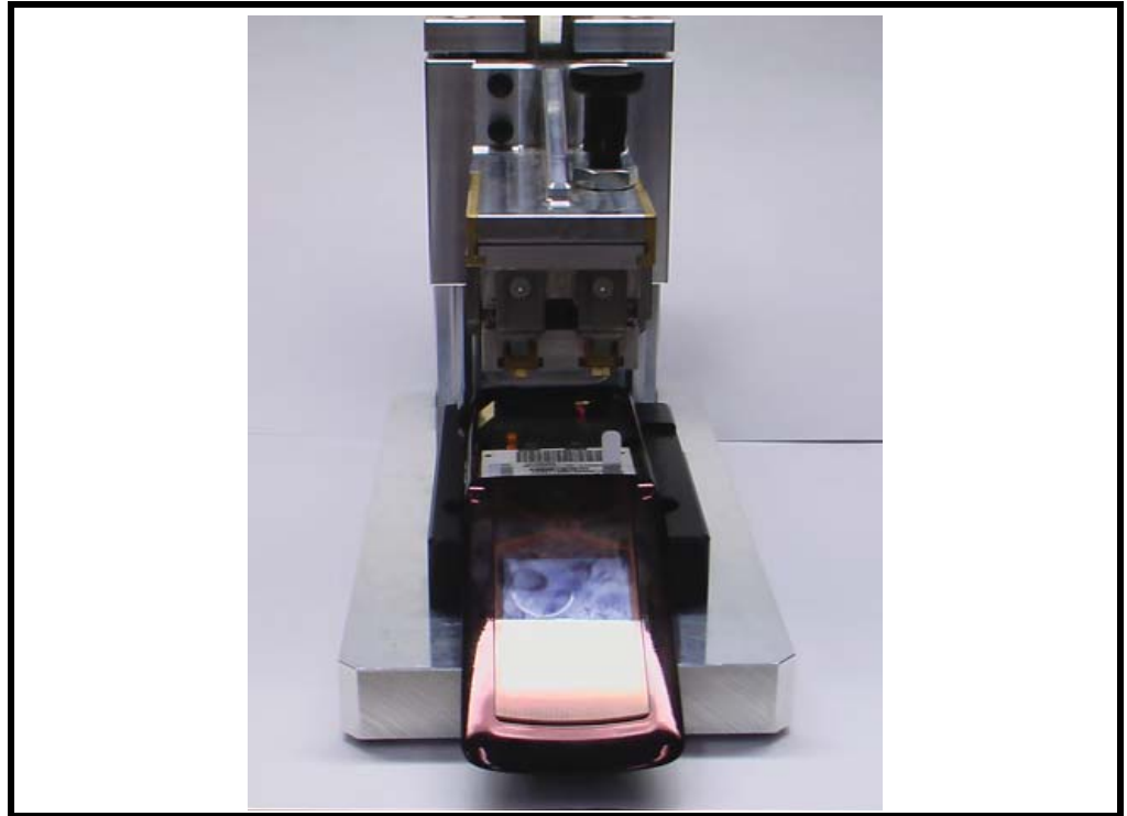
Figure 26. Keypad Tab Bend Fixture
