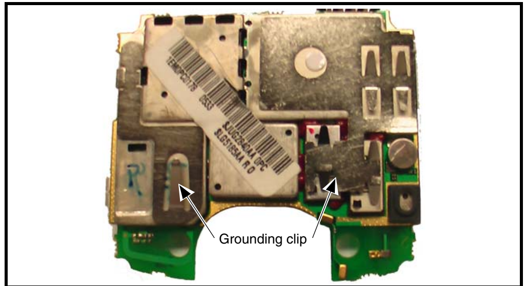
Figure 15. Transceiver PC board Assembly Grounding Clip
