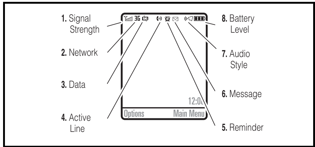
Figure 3. Icon Indicators
