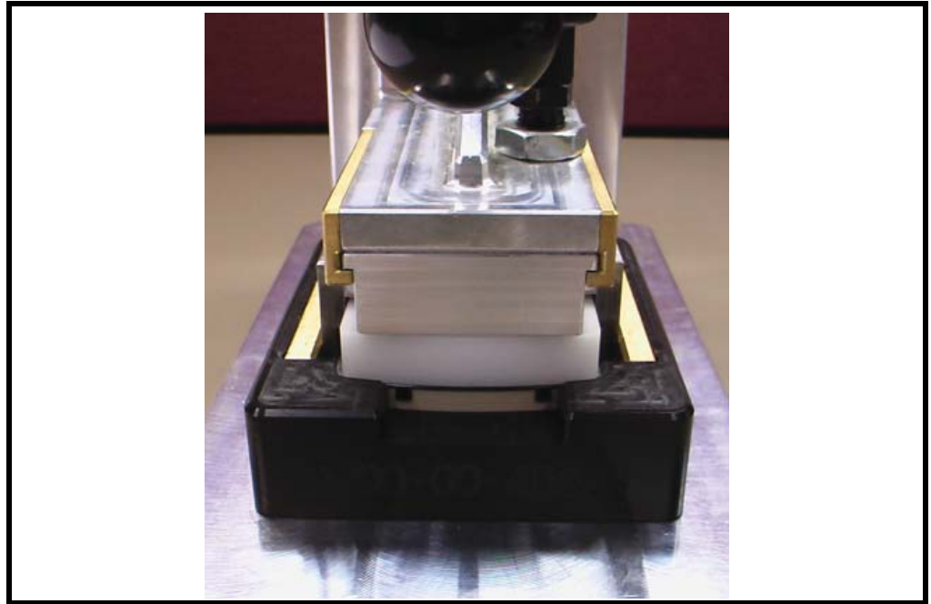
Figure 23. Keypad Side Tab Bend Fixture Closed
