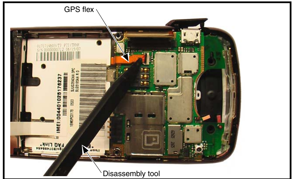
Figure 13. Releasing the GPS Flex Connector (North America Region only)
