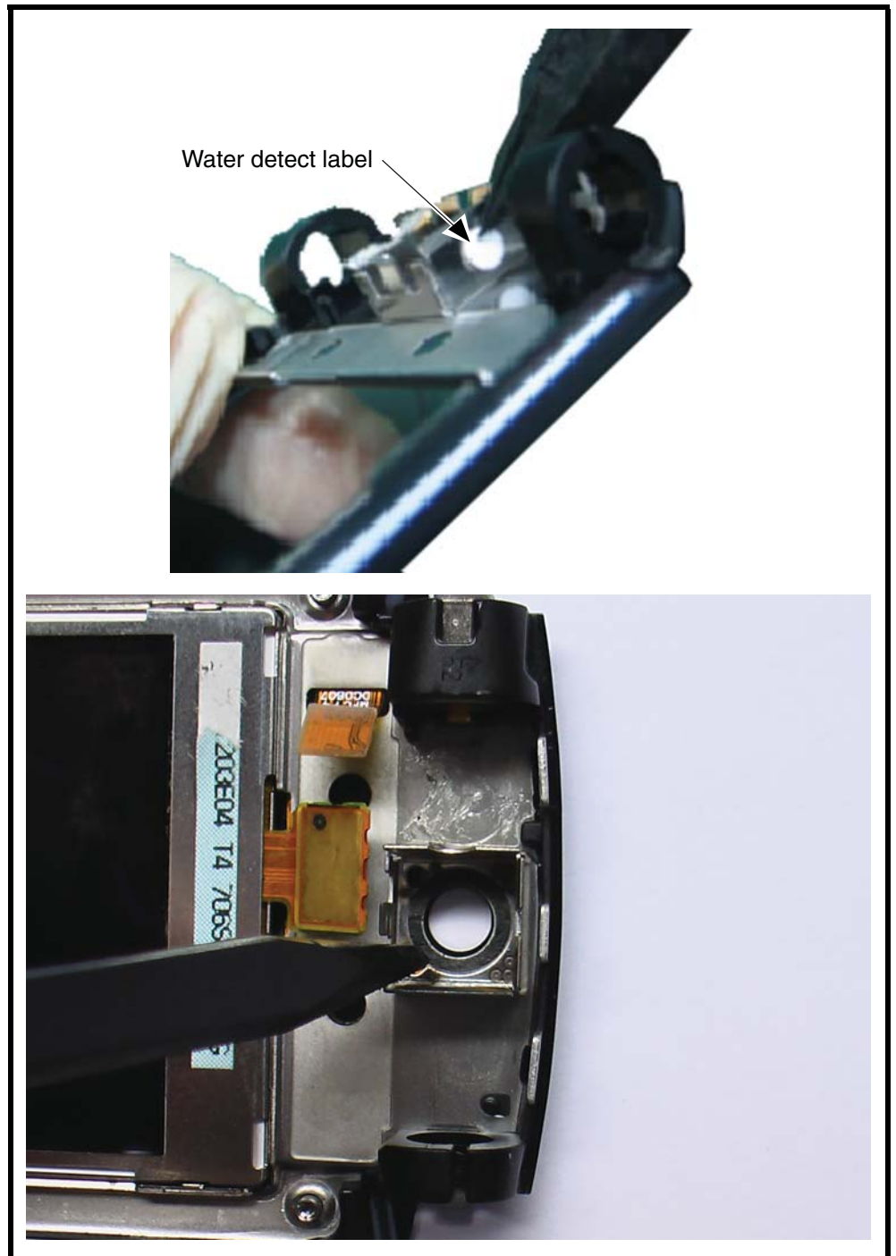
Figure 57. Installing the Water Label
