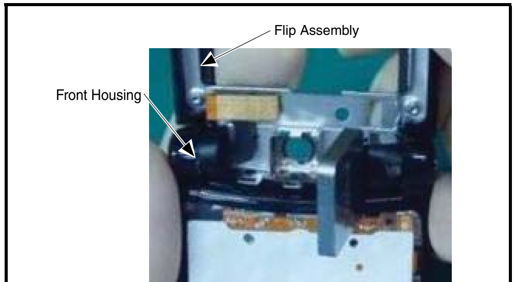
Figure 61. Aligning the Flip Assembly to the Front Housing
