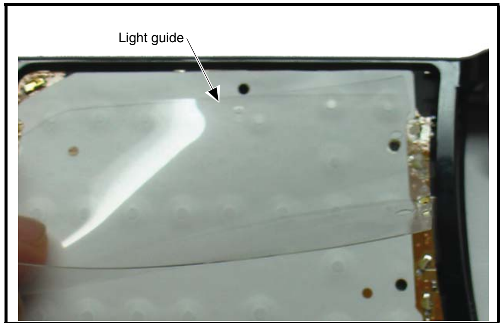
Figure 41. Removing the Light Guide
