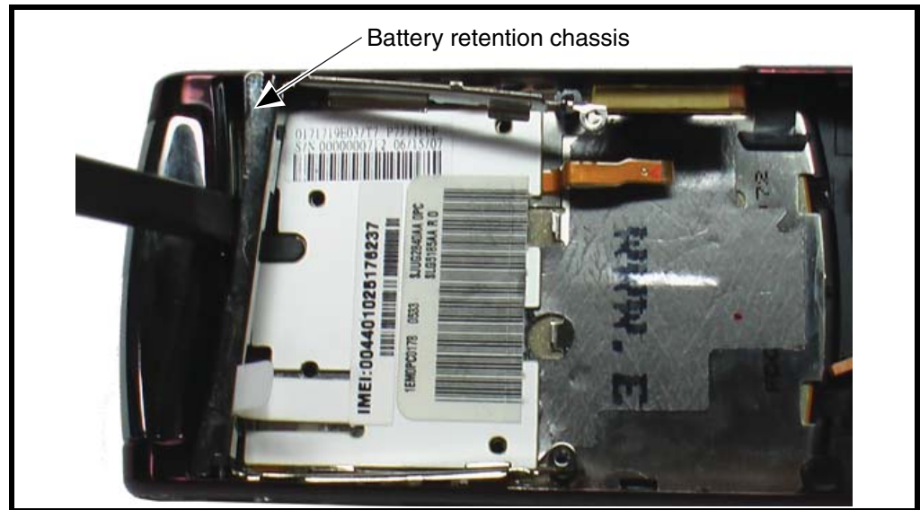
Figure 20. Removing the Battery Retention Chassis
