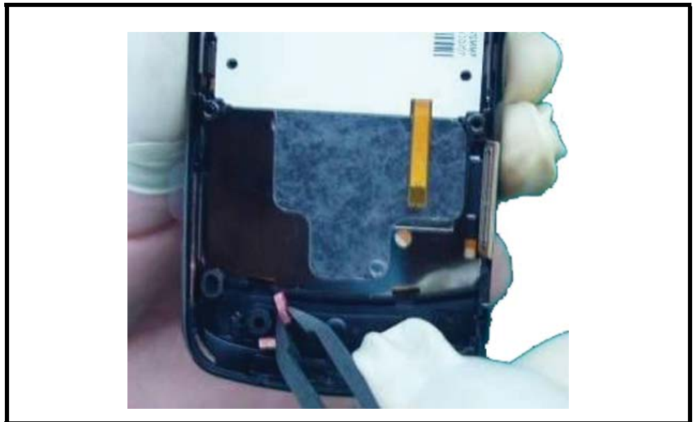
Figure 84. installing Speaker Contacts
