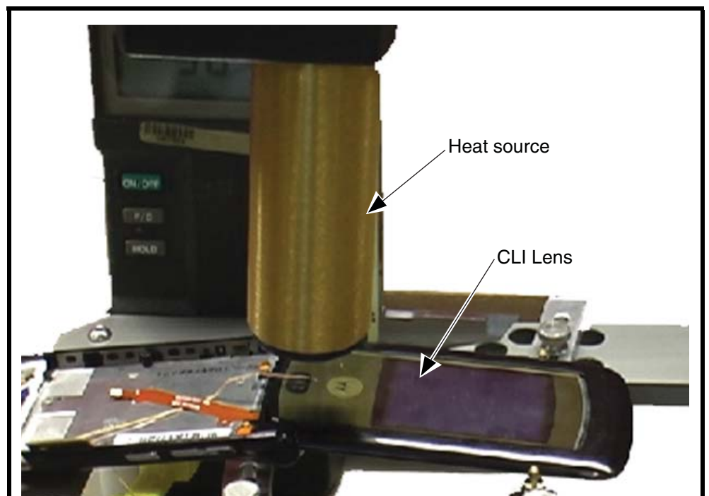
Figure 31. Heating the CLI Lens
