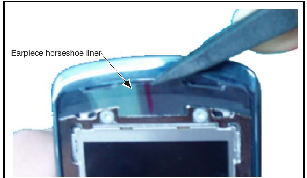
Figure 79. Removing the Earpiece Horseshoe Liner
