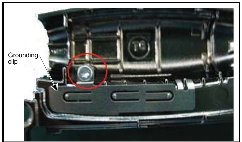
Figure 76. Installing Grounding Clip
