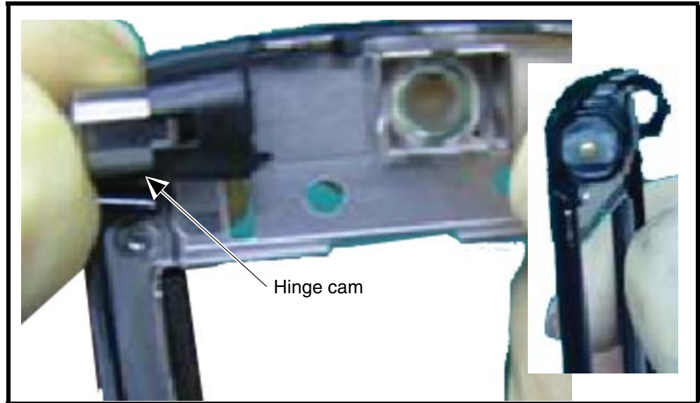
Figure 58. Installing the Flip Hinge Cam
