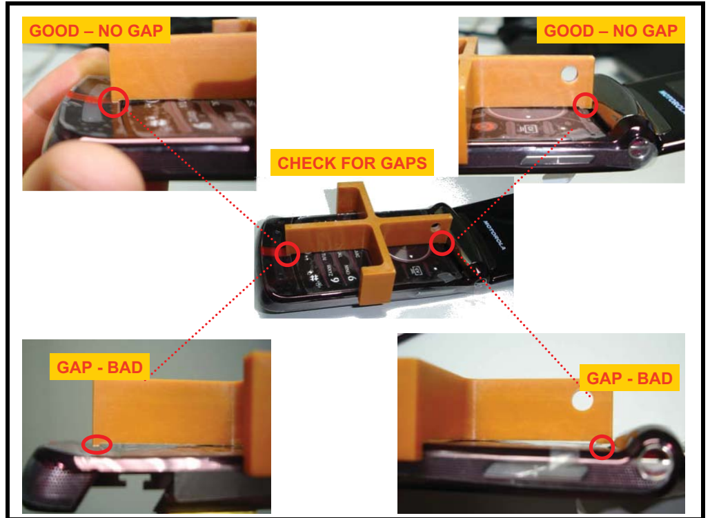
Figure 28. Keypad Bow Test
