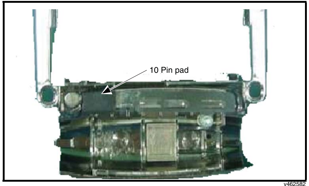
Figure 75. installing 10 Pin Pad
