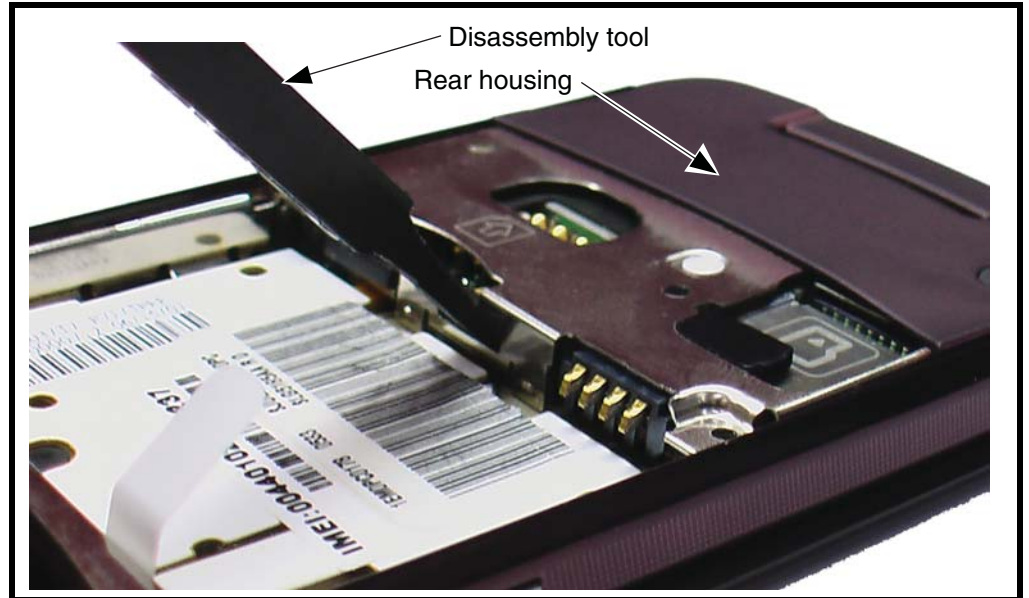
Figure 7. Removing the Rear Housing Latches
