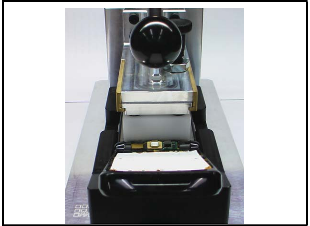
Figure 70. CLI Lens Press Fixture Opened
