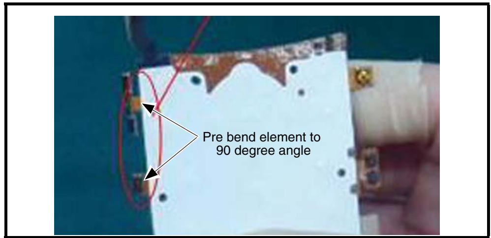
Figure 48. Bending the K Flex Left Element
