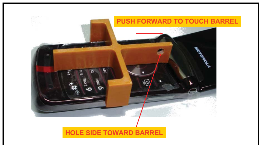
Figure 27. Keypad Bow Test
