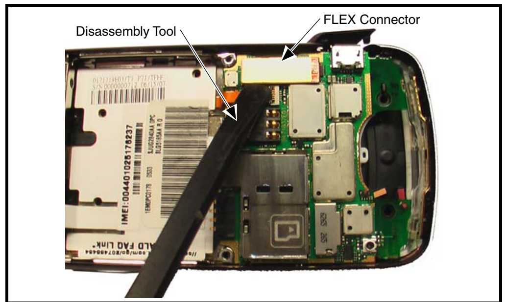
Figure 12. Unseating the Flex Connector
