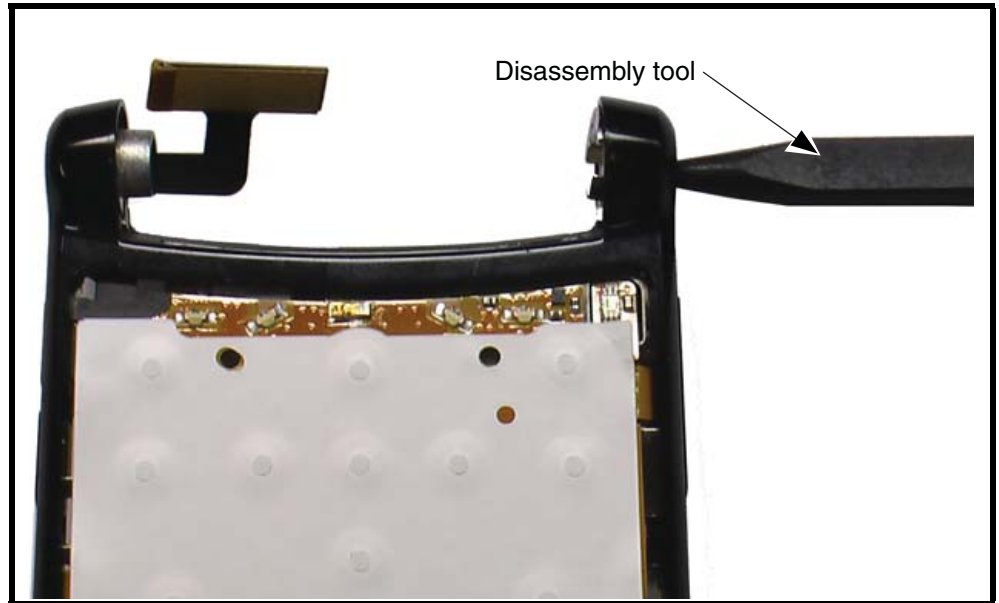
Figure 42. Removing the Lanyard Collar
