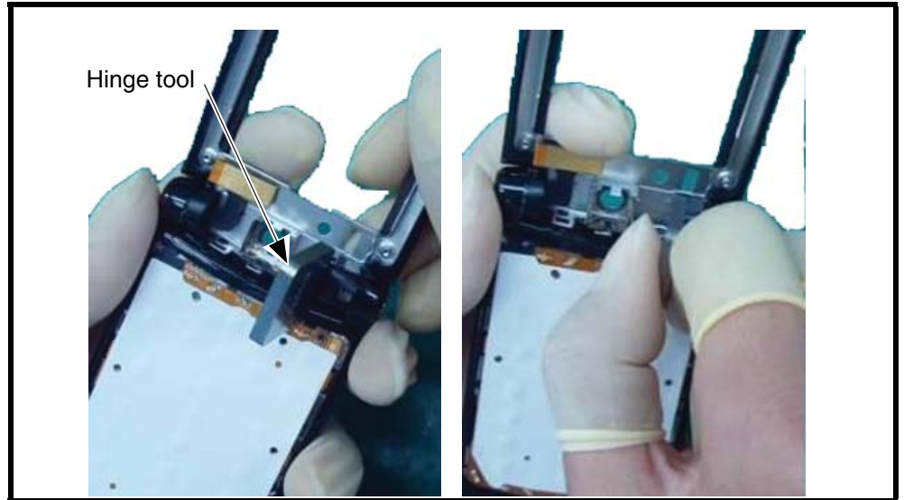
Figure 40. Removing the Flip Hinge
