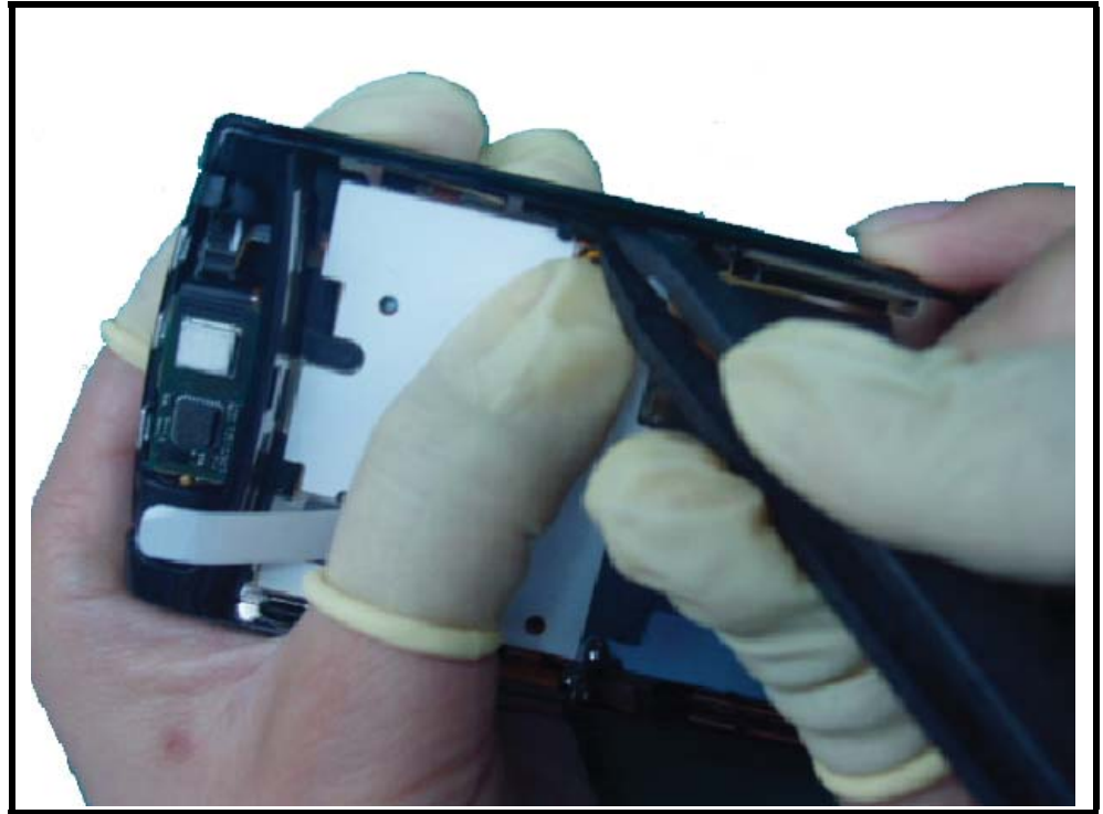
Figure 56. Installing the Side Key
