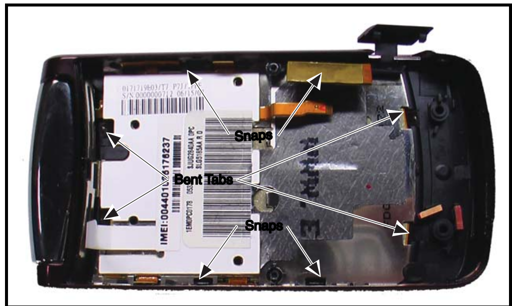
Figure 21. Location of Keypad Tabs and Snaps
