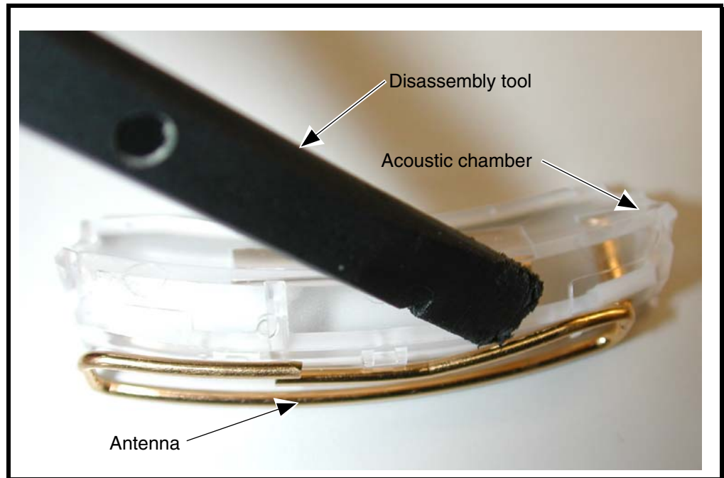
Figure 12. Removing the Antenna
