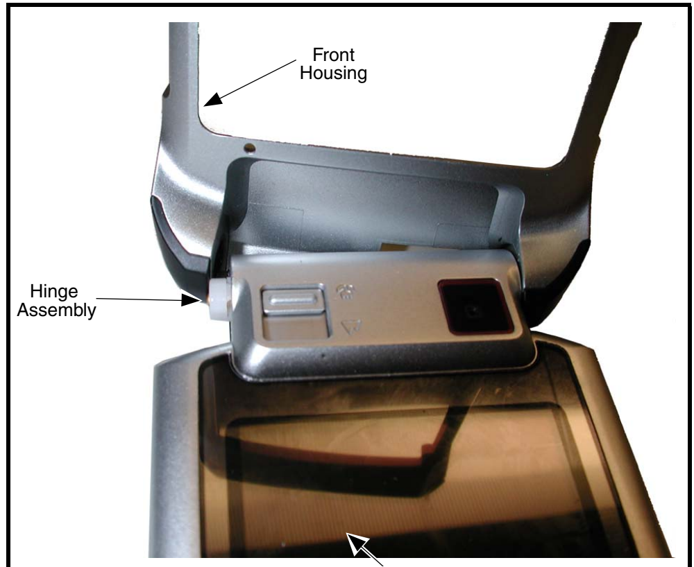
Figure 15. Removing the Flip Assembly
