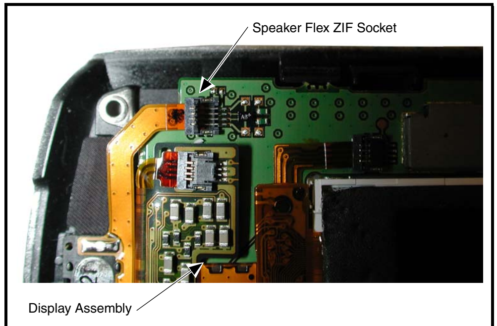
Figure 22. Removing the Display Assembly Flex Connector
