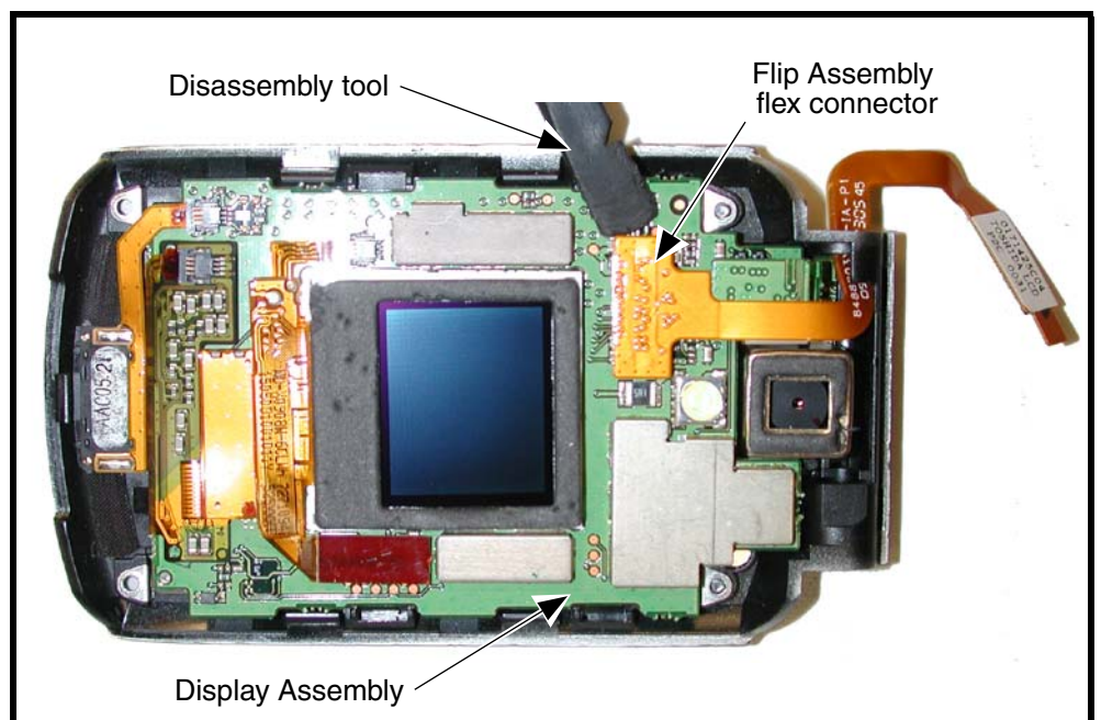
Figure 20. Removing the Flip Assembly Flex Connector
