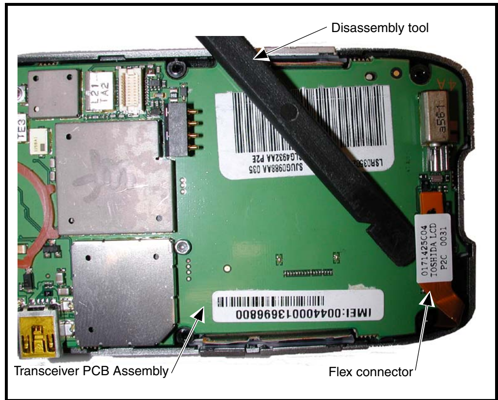
Figure 7. Disconnecting the Flex From the Transceiver Board
