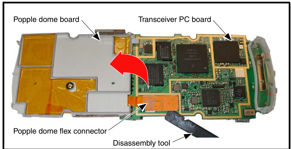
Figure 10. Removing the Popple dome FLEX Connector
