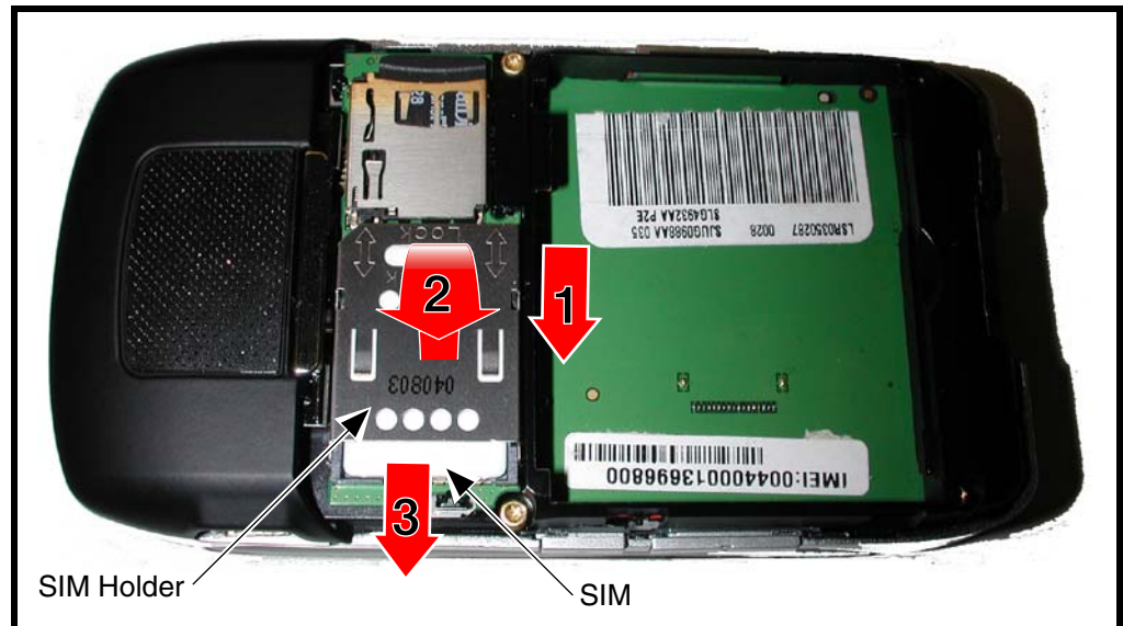
Figure 3. Removing the SIM
