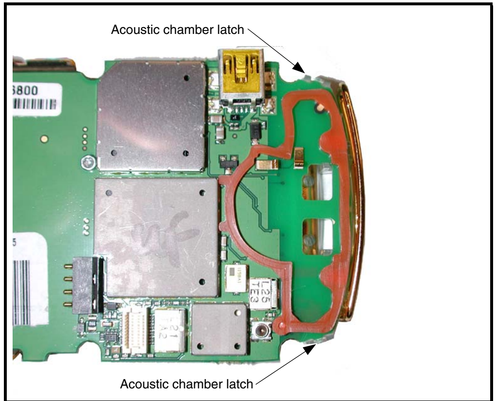
Figure 11. Removing the Antenna Assembly
