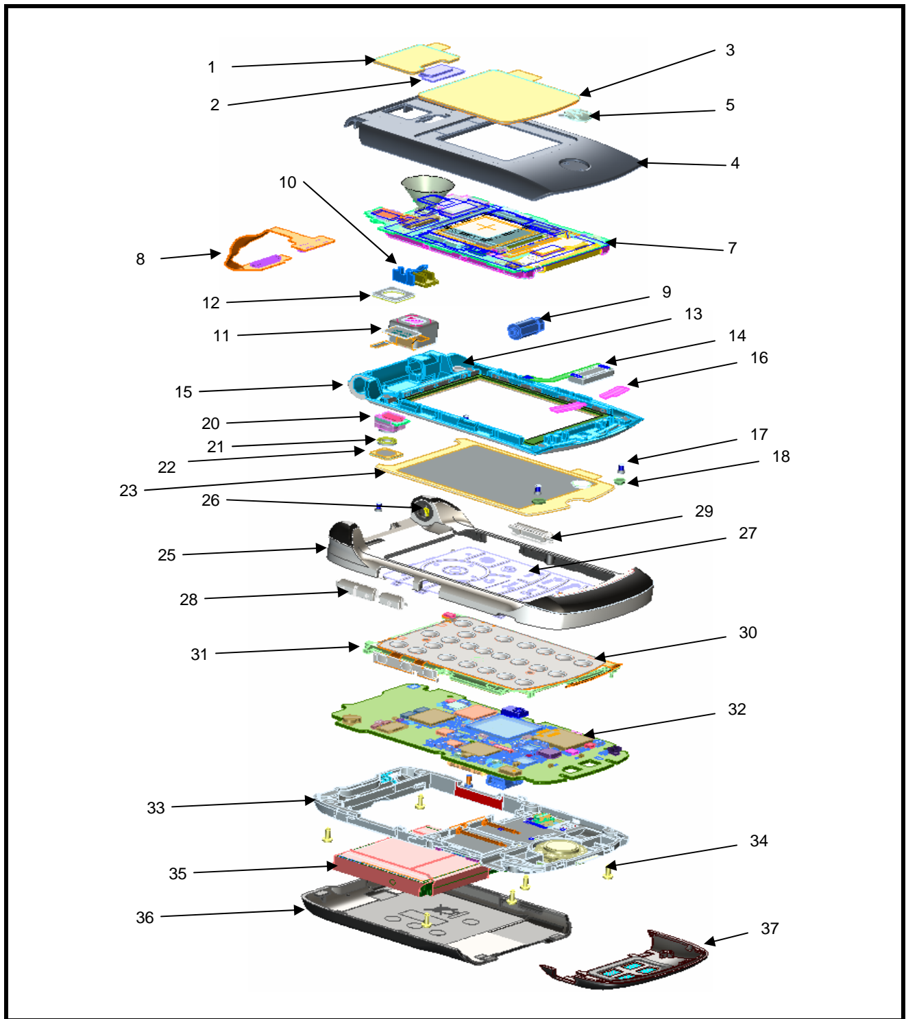
Figure 25. Exploded View Diagram
