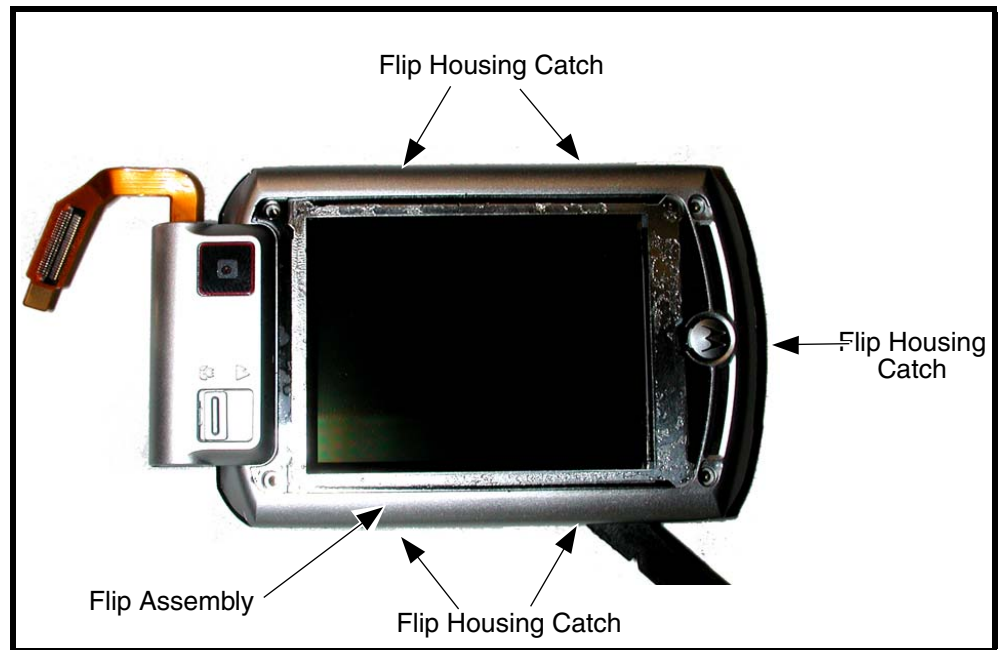
Figure 19. Removing the Display Lens
