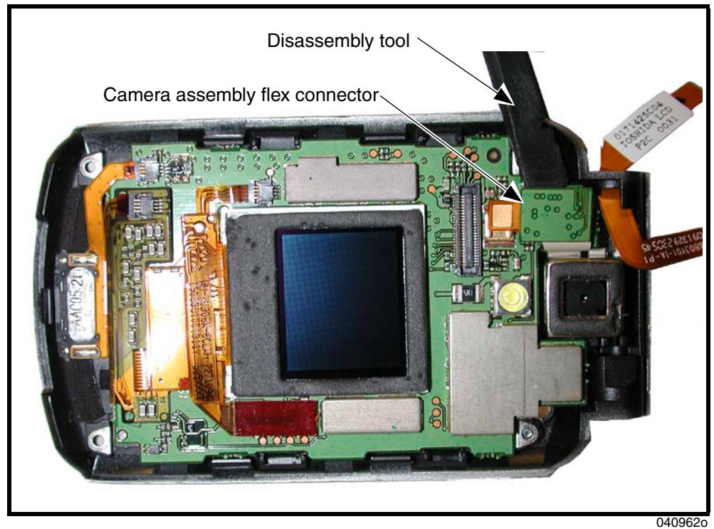
Figure 21. Removing the Camera Assembly Flex Connector
