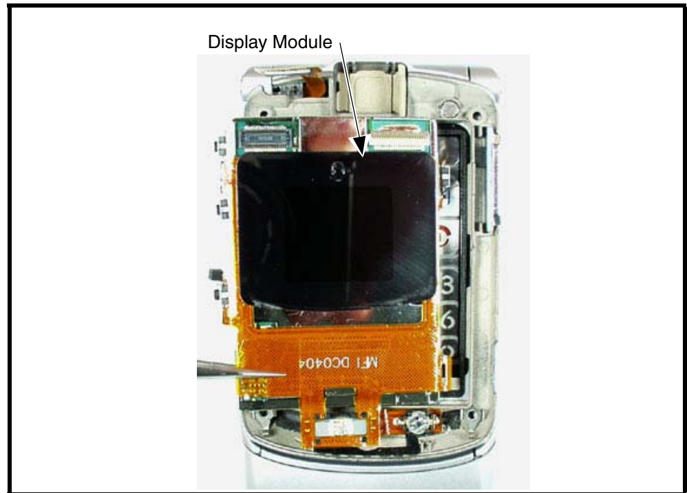
Figure 15. Removing the Display Module Assembly
