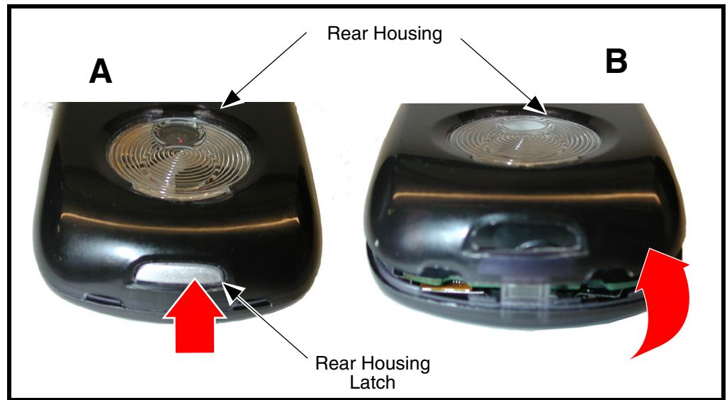
Figure 4. Removing the Rear housing Cover
