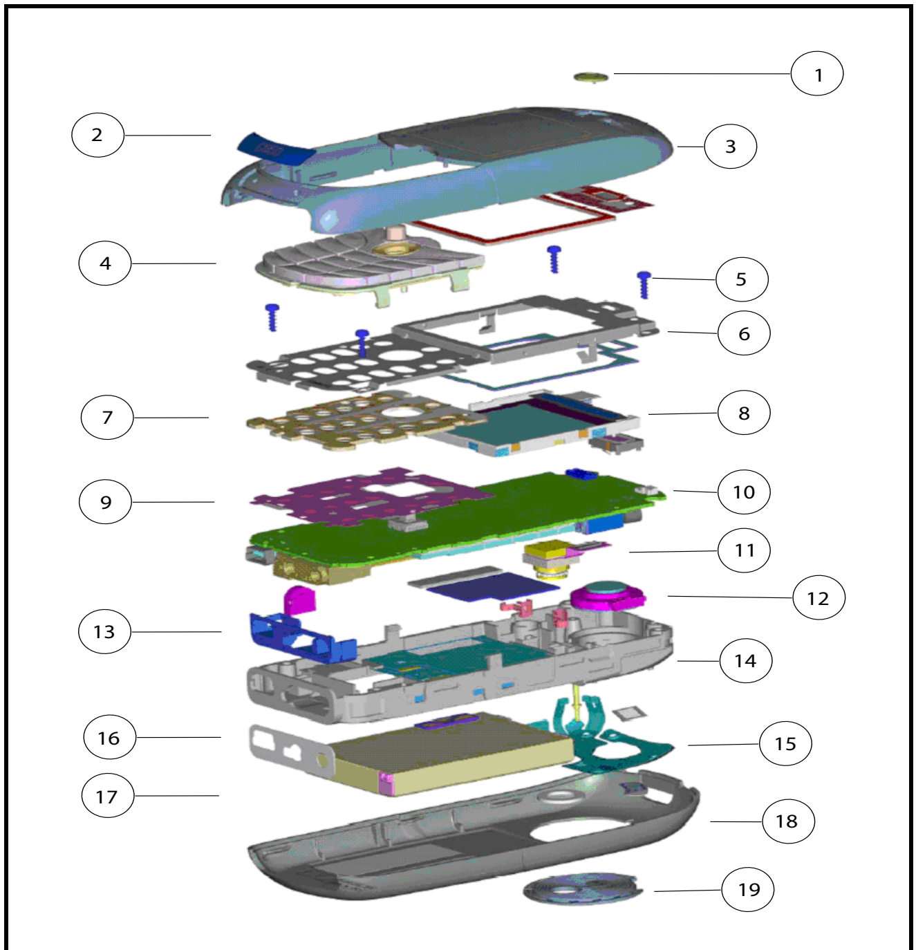
Figure 16. Exploded View Diagram
