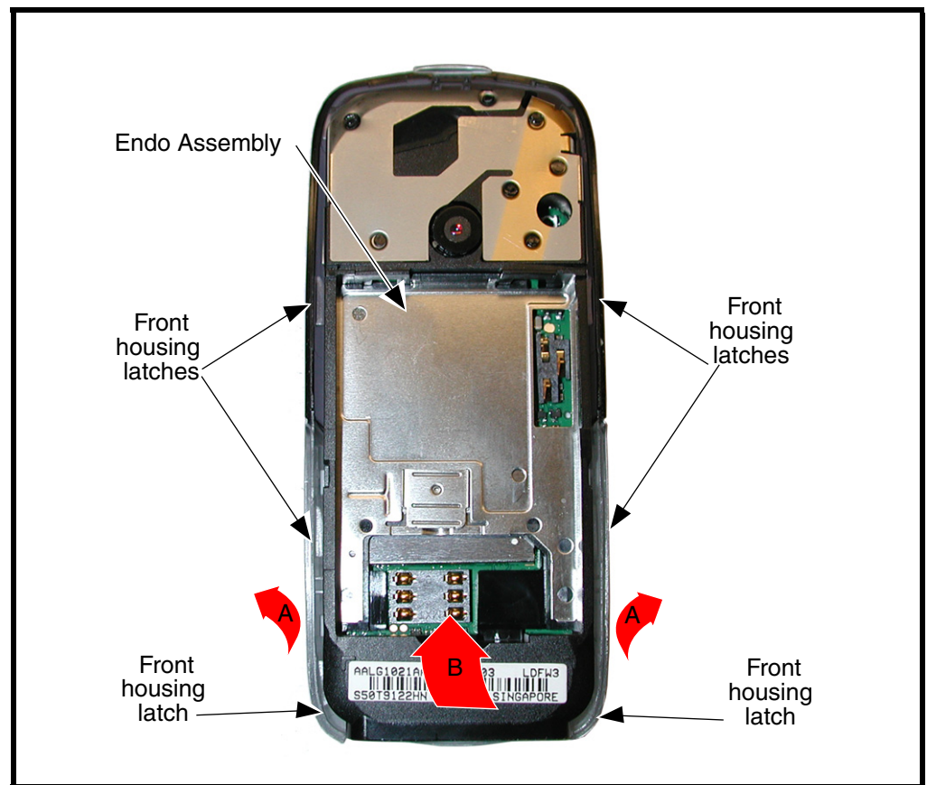
Figure 7. Removing the Endo Assembly
