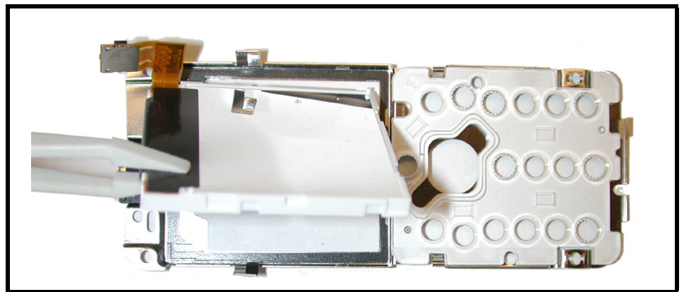
Figure 13. Removing the Display Assembly
