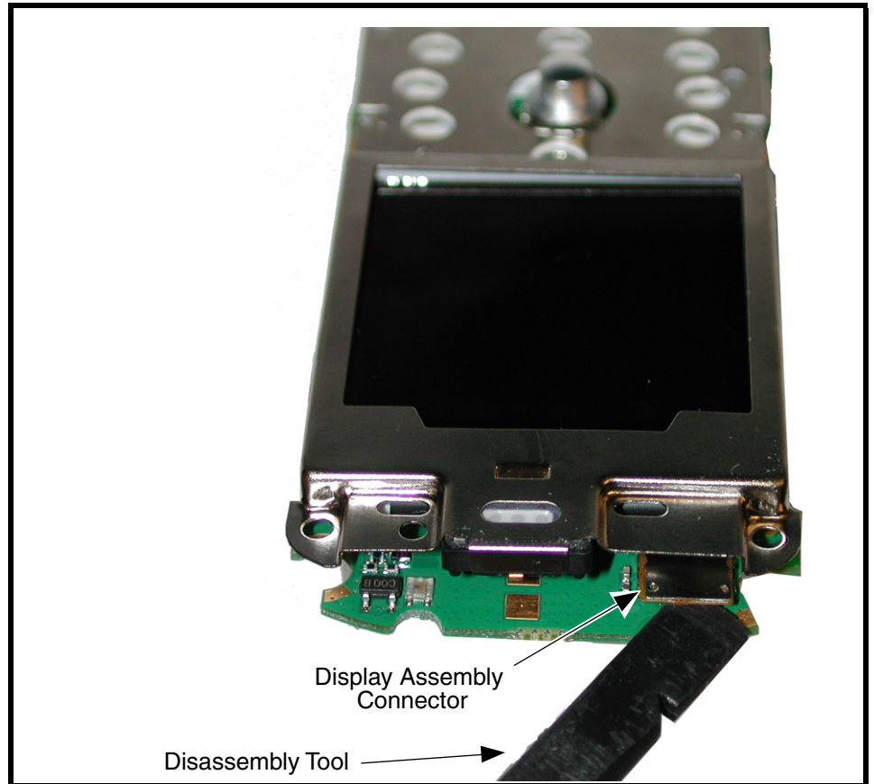
Figure 12. Removing the Display Assembly Connector
