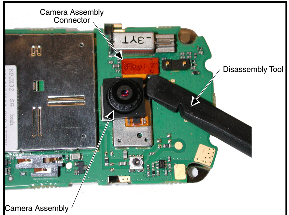
Figure 10. Removing the Camera Assembly
