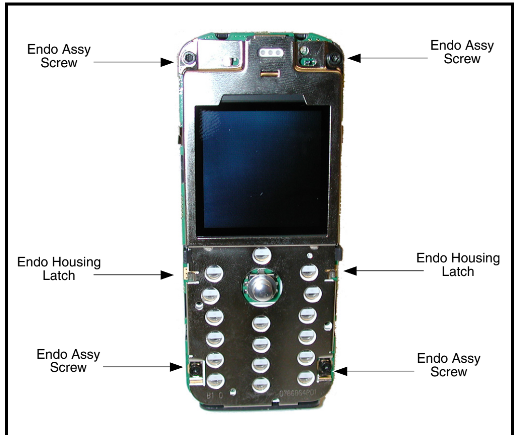
Figure 9. Removing the Front Endo Assembly
