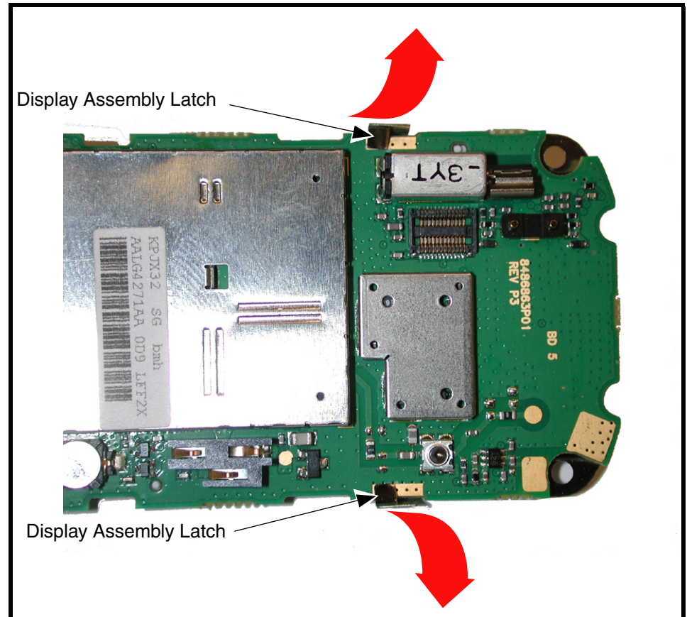
Figure 11. Removing the Display Assembly Latches
