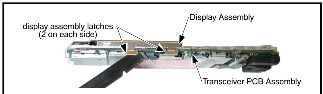
Figure 14. Removing the Transceiver Board
