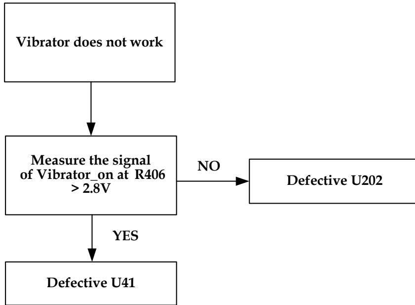
Faulting Finding Chart of "Vibrator failed"
