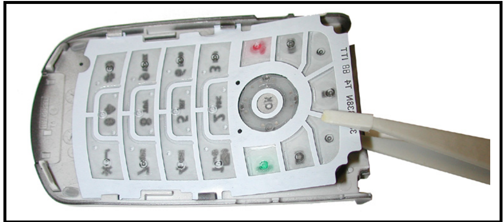
Figure 25. Removing the Keypad
