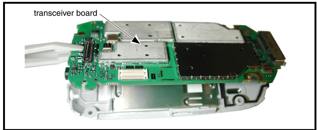
Figure 19. Removing the Transceiver Board
